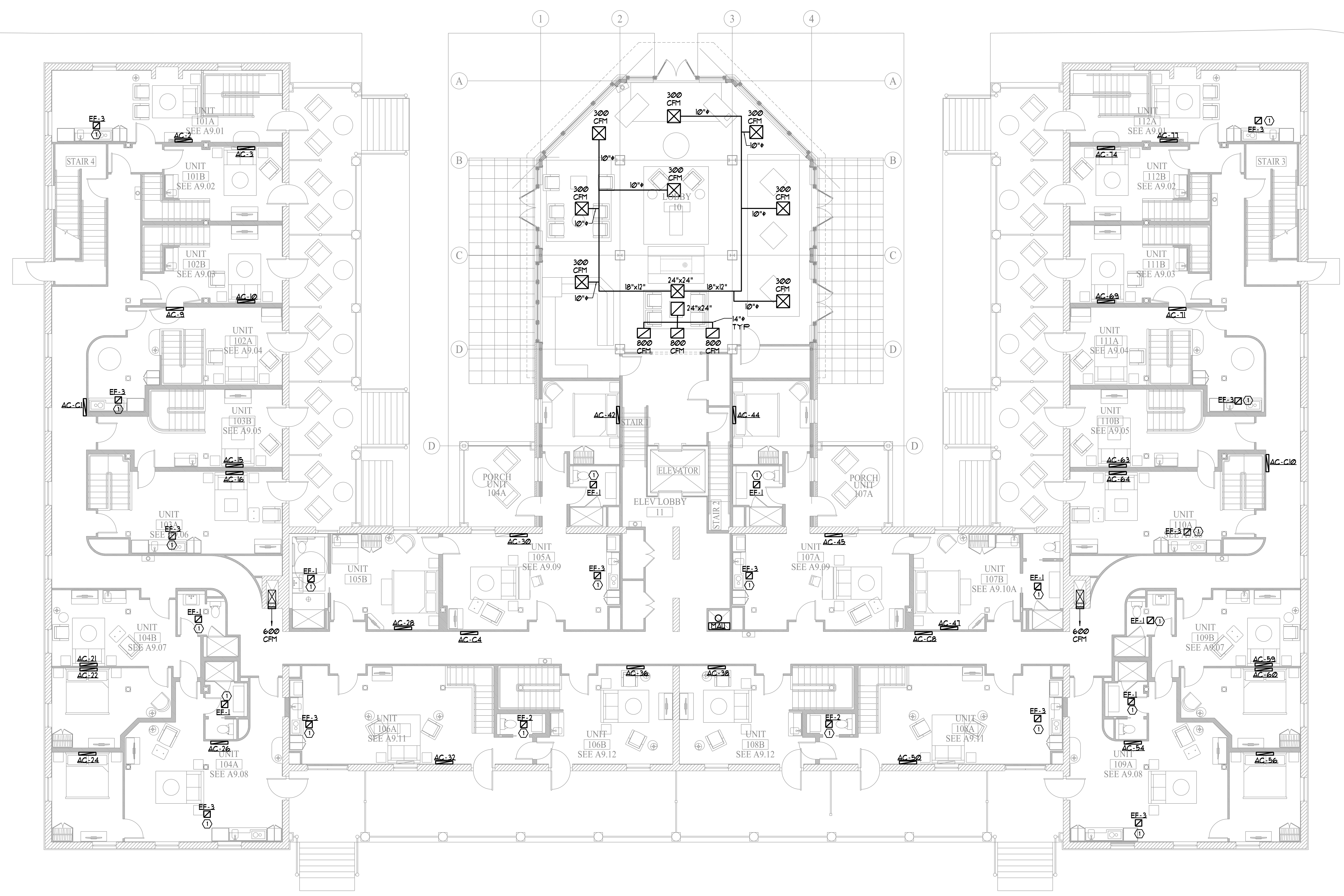
FIRST FLOOR MECHANICAL PLAN SCALE 1/8" = 1'-0"
