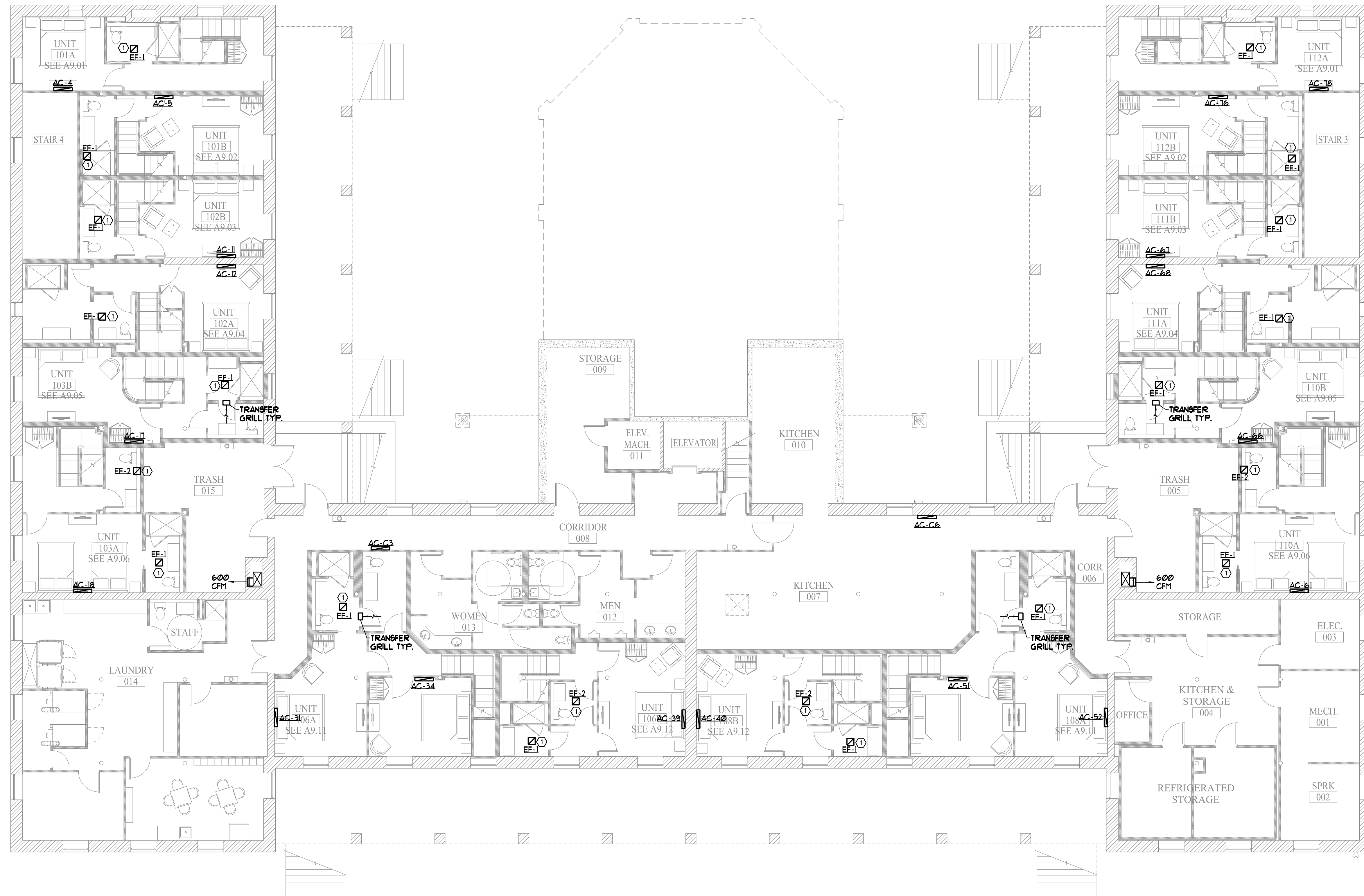
BASEMENT MECHANICAL PLAN SCALE 1/8" = 1'-0"
