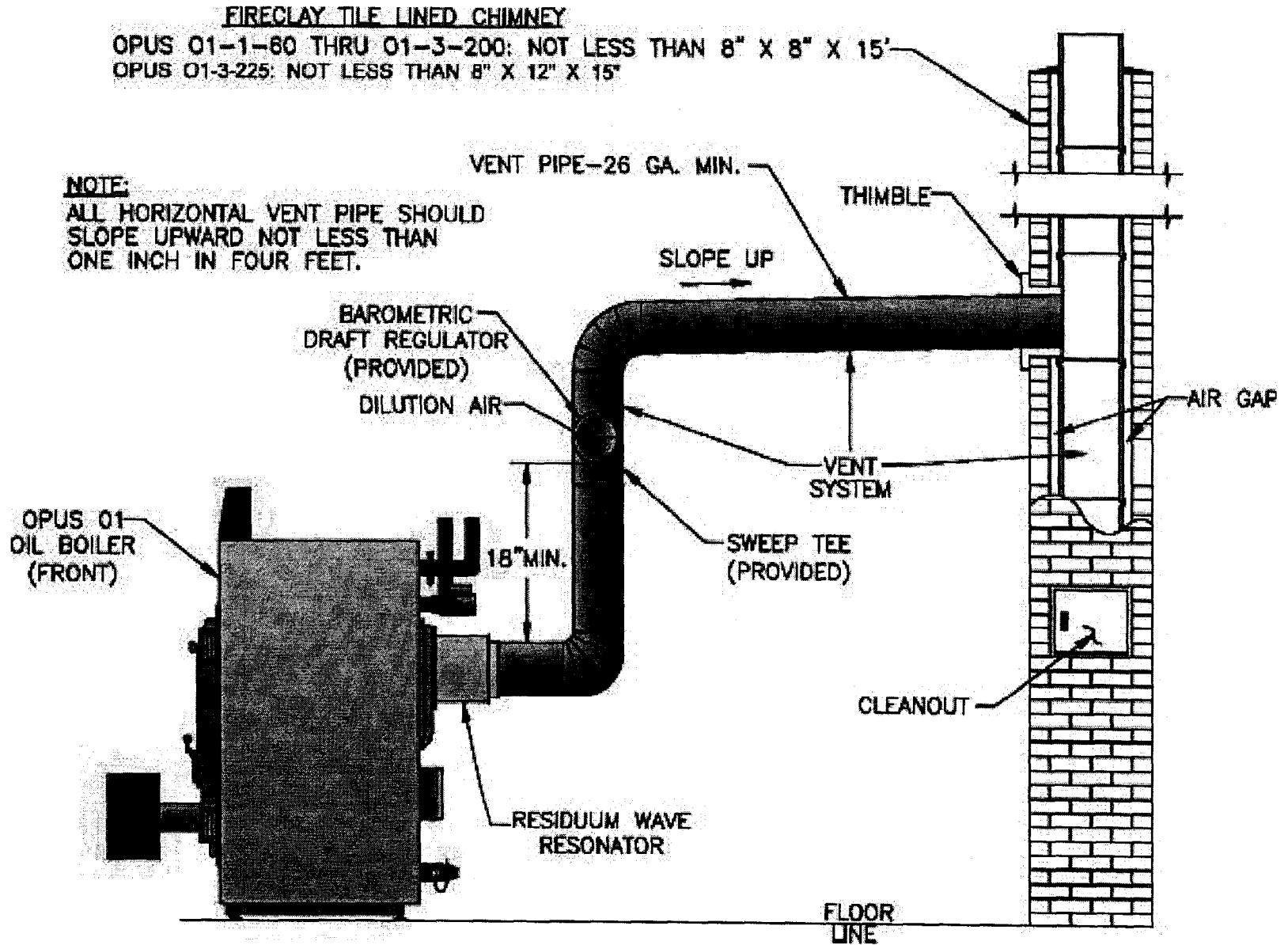
Figure 10: Recommended Vent Pipe Arrangement and Chimney Requirements
