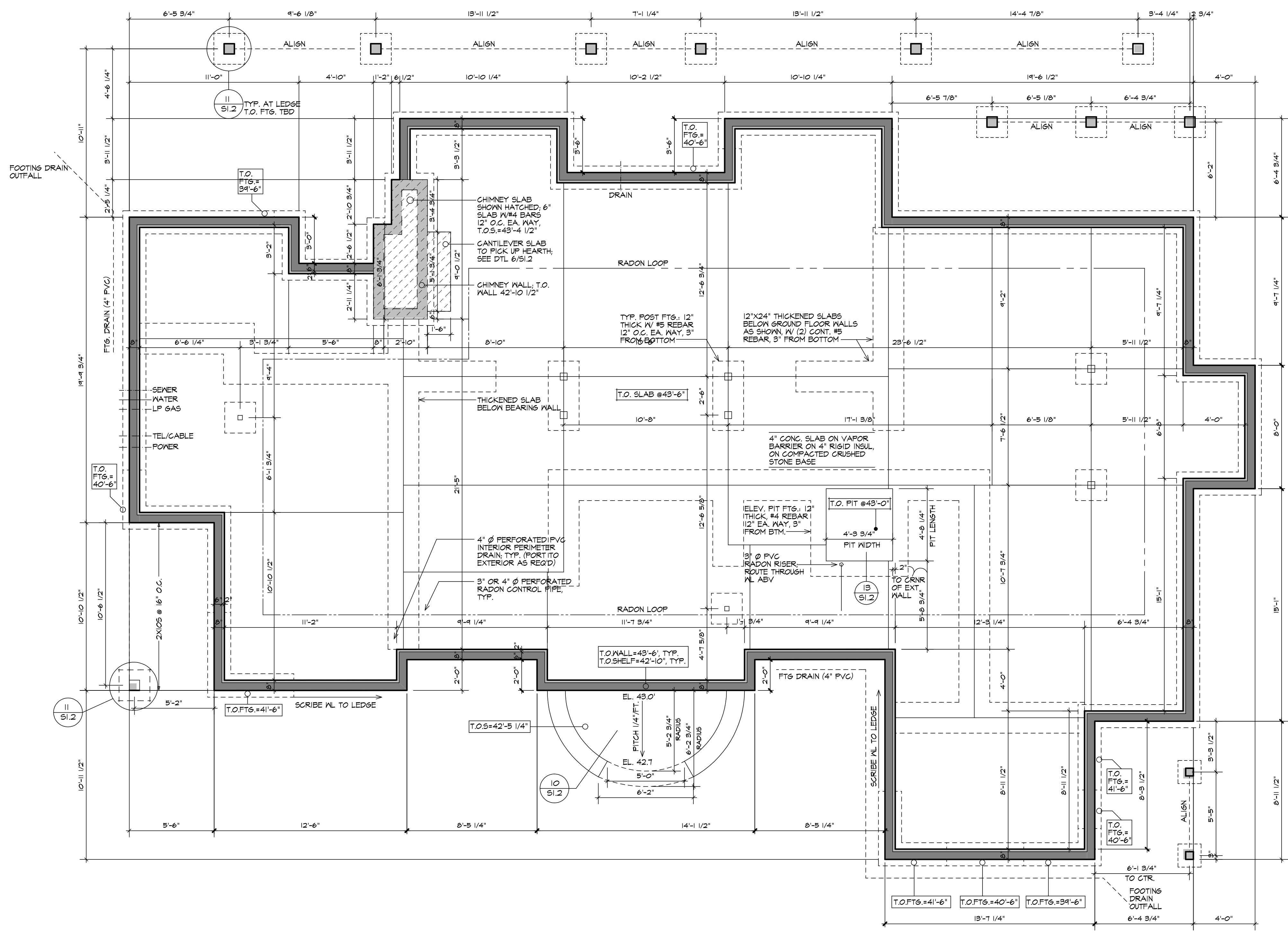
FOUNDATION PLAN S1.1 1/4" = 1'-0"
