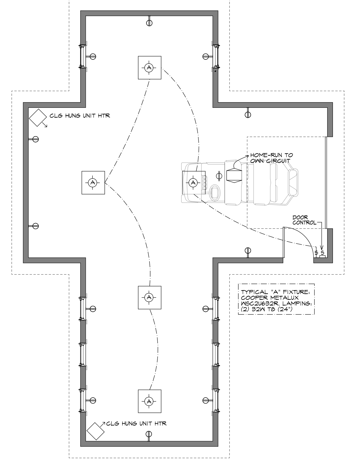
3 GARAGE ELECTRICAL PLAN A10.1 1/4" = 1'-0"
