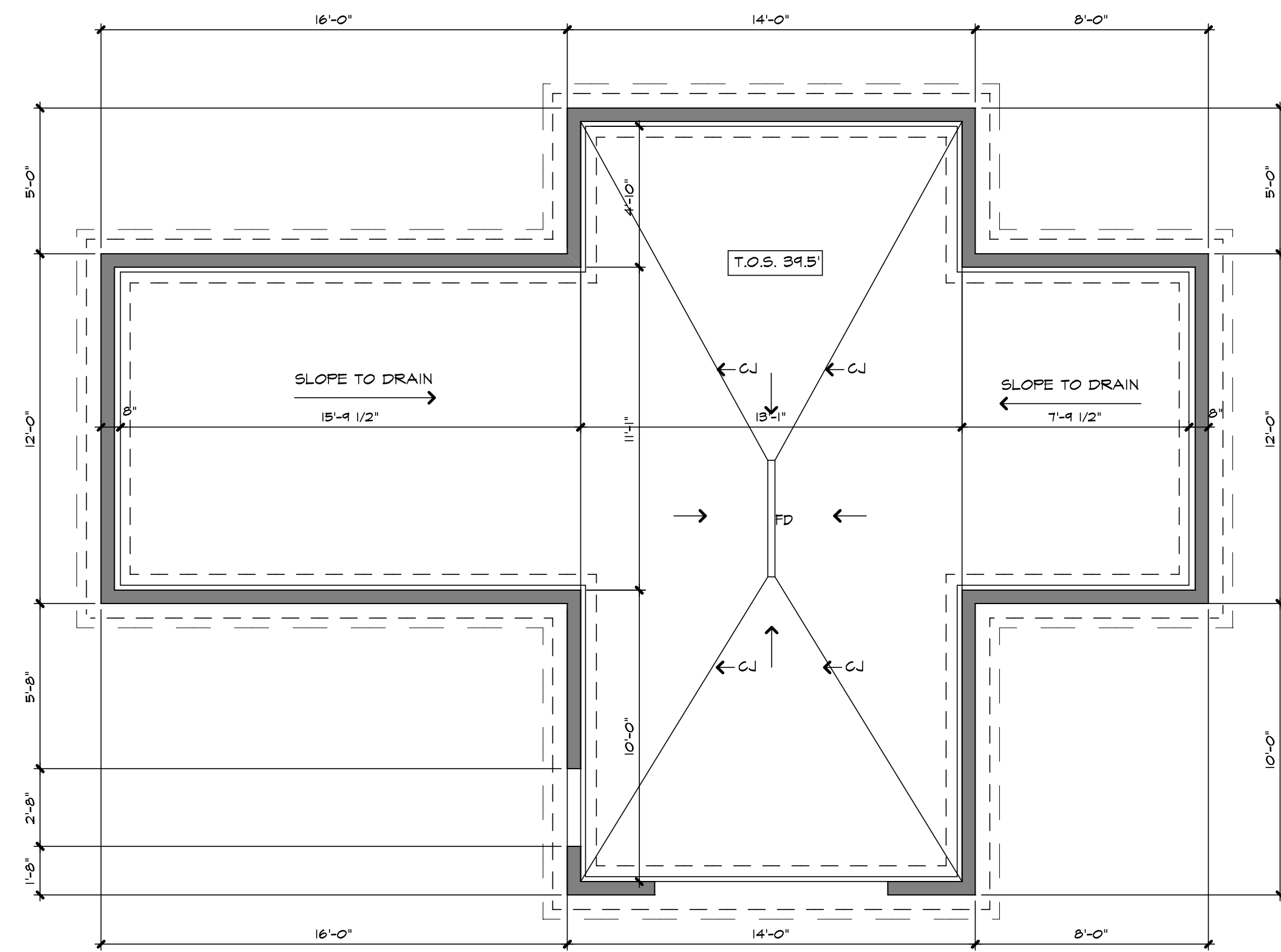
2 GARAGE FOUNDATION PLAN A10.1 1/4" = 1'-0"
