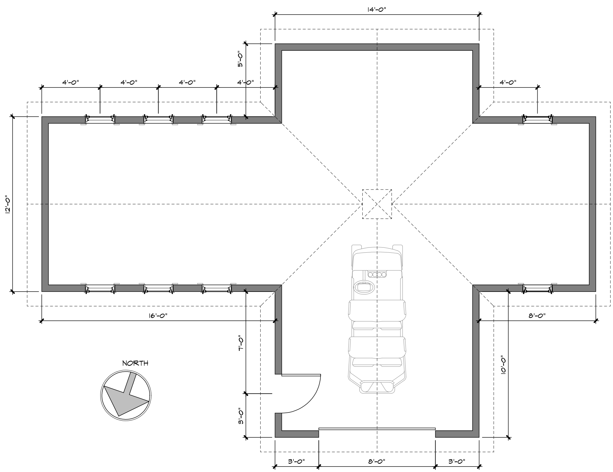
1 GARAGE FLOOR PLAN A10.1 1/4" = 1'-0"
