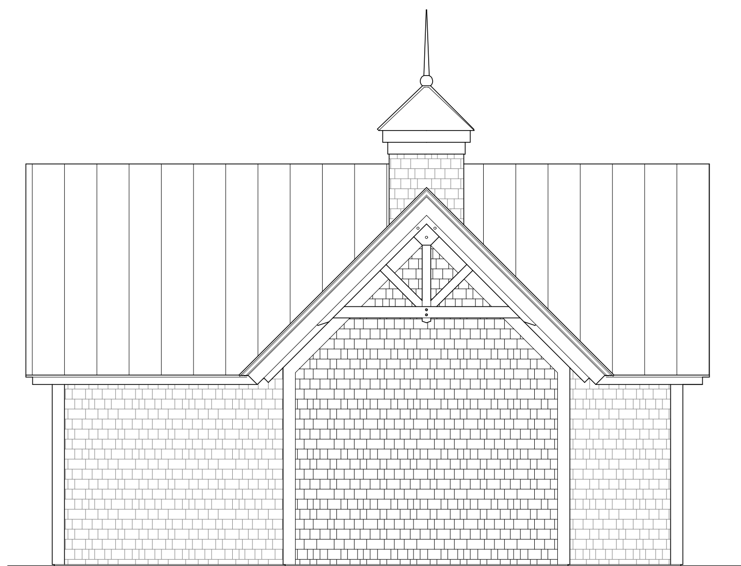
5 GARAGE: WEST ELEVATION A10.1 1/4" = 1'-0"
