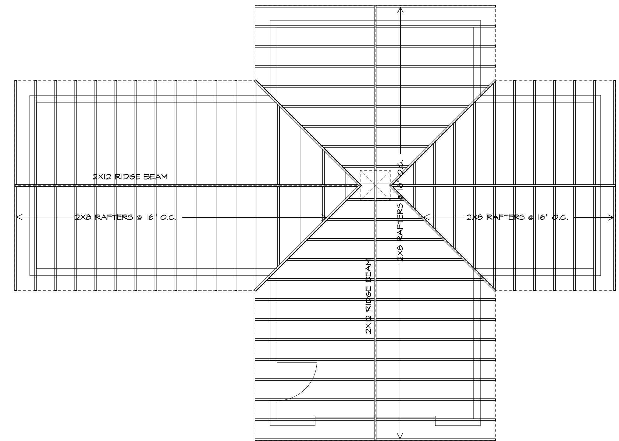
1 GARAGE FRAMING PLAN A10.1 1/4" = 1'-0"
