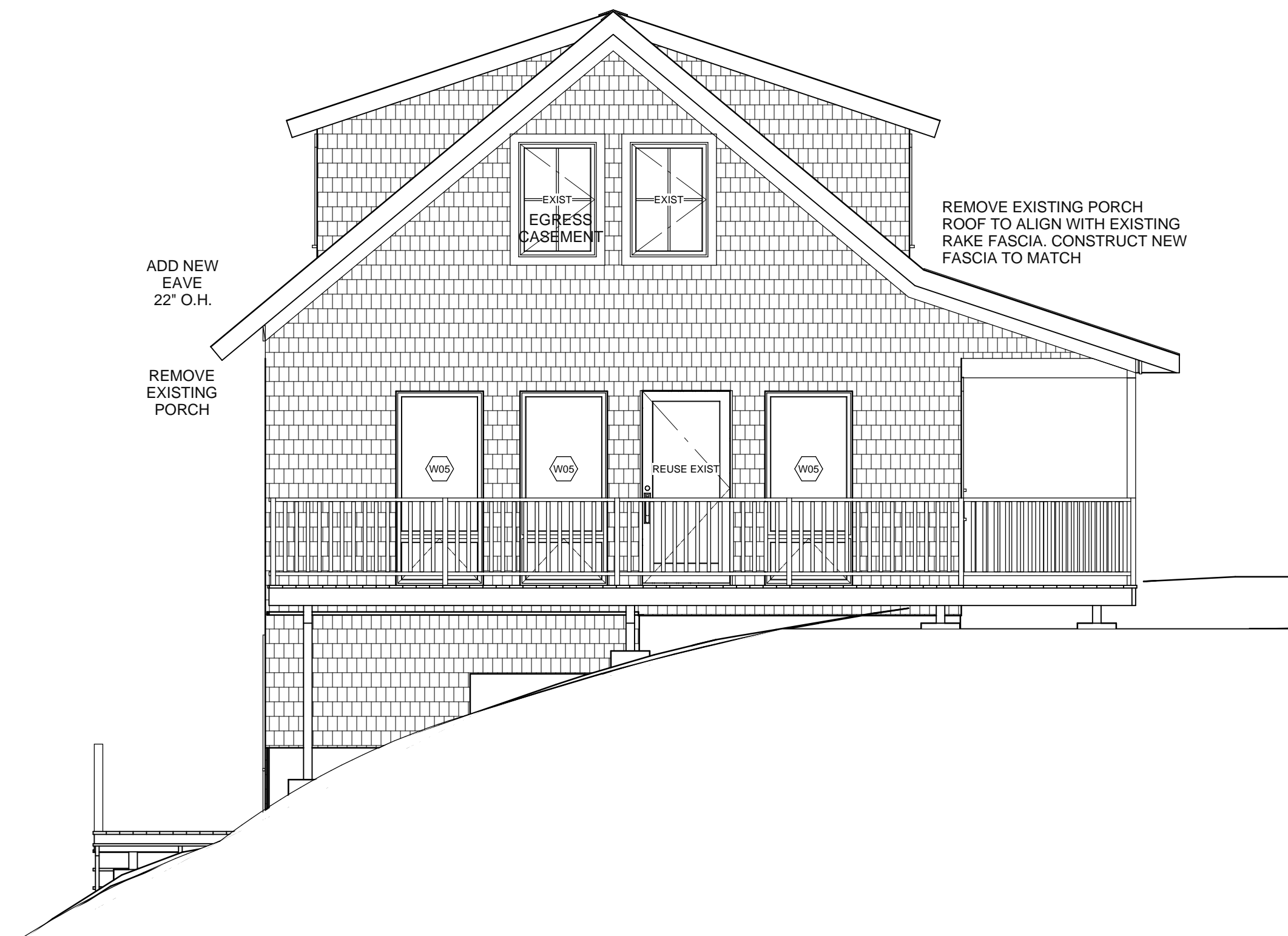
South Elev
