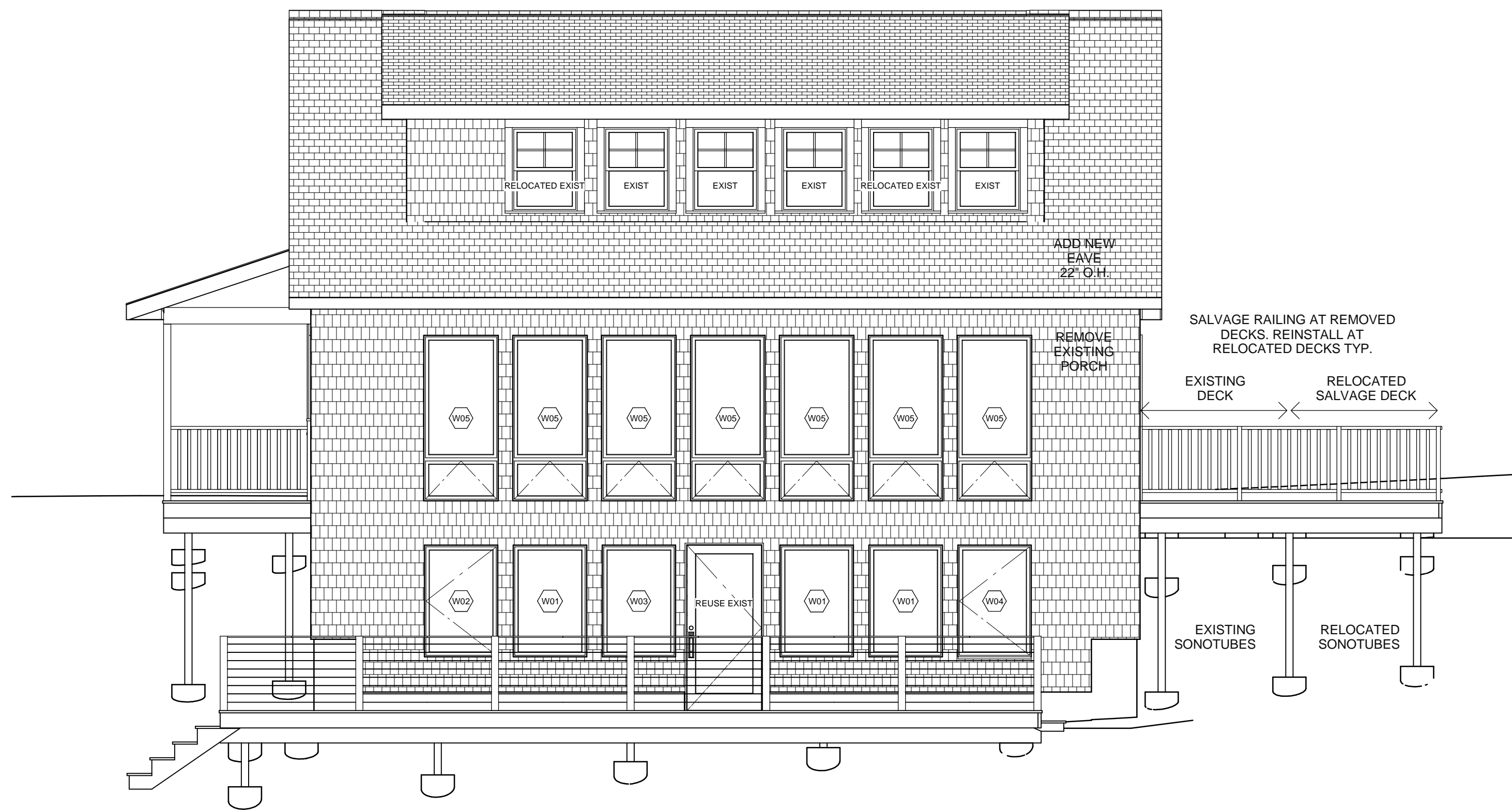
East Elev
