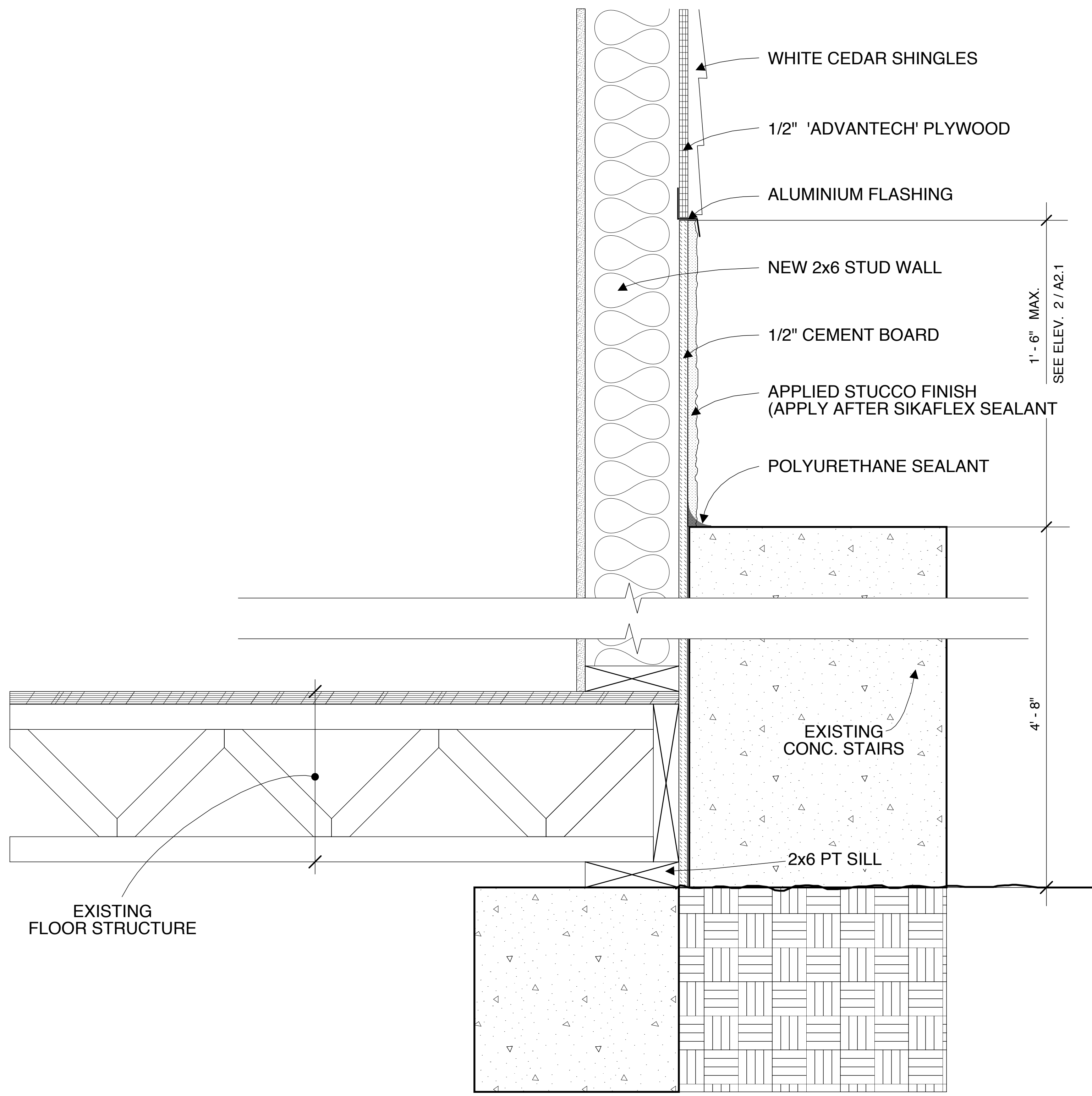
1 WALL REPAIR DETAIL SCALE: 3" = 1'-0"
