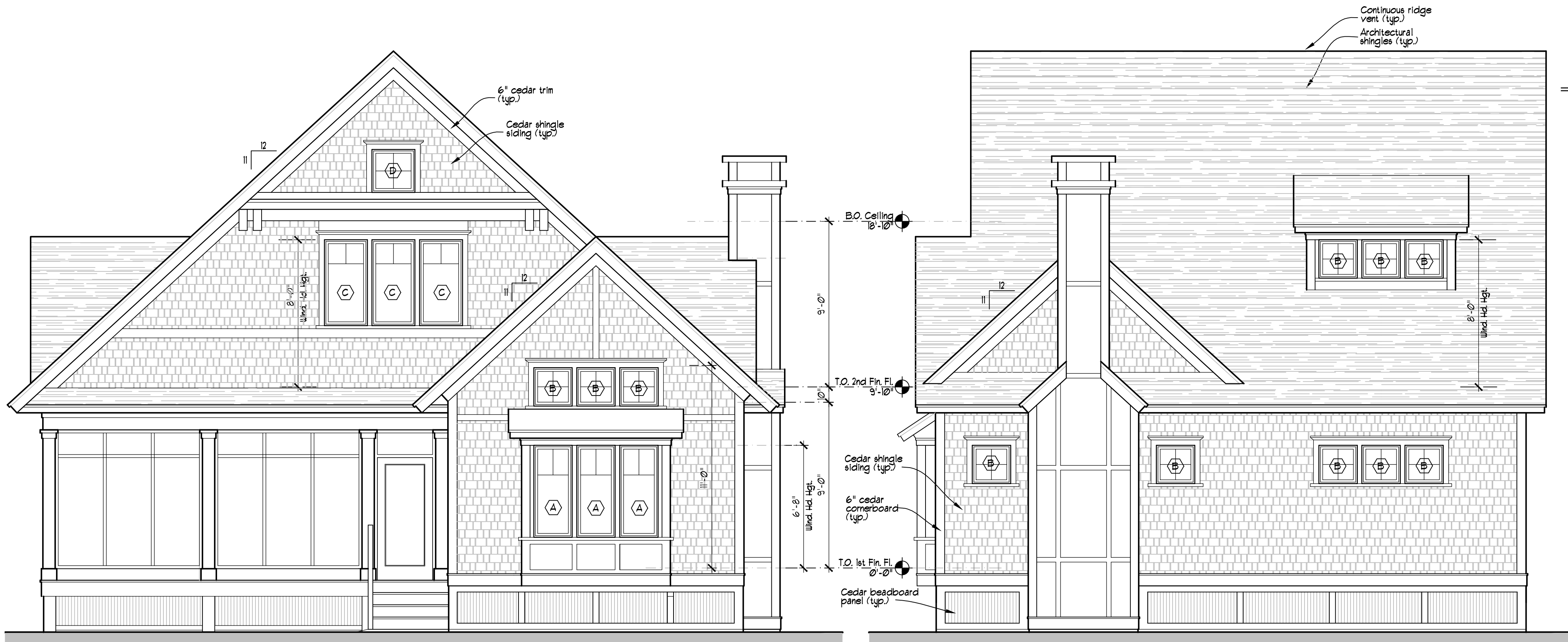
2 FRONT ELEVATION SCALE: 1/4" = 1'-0"
