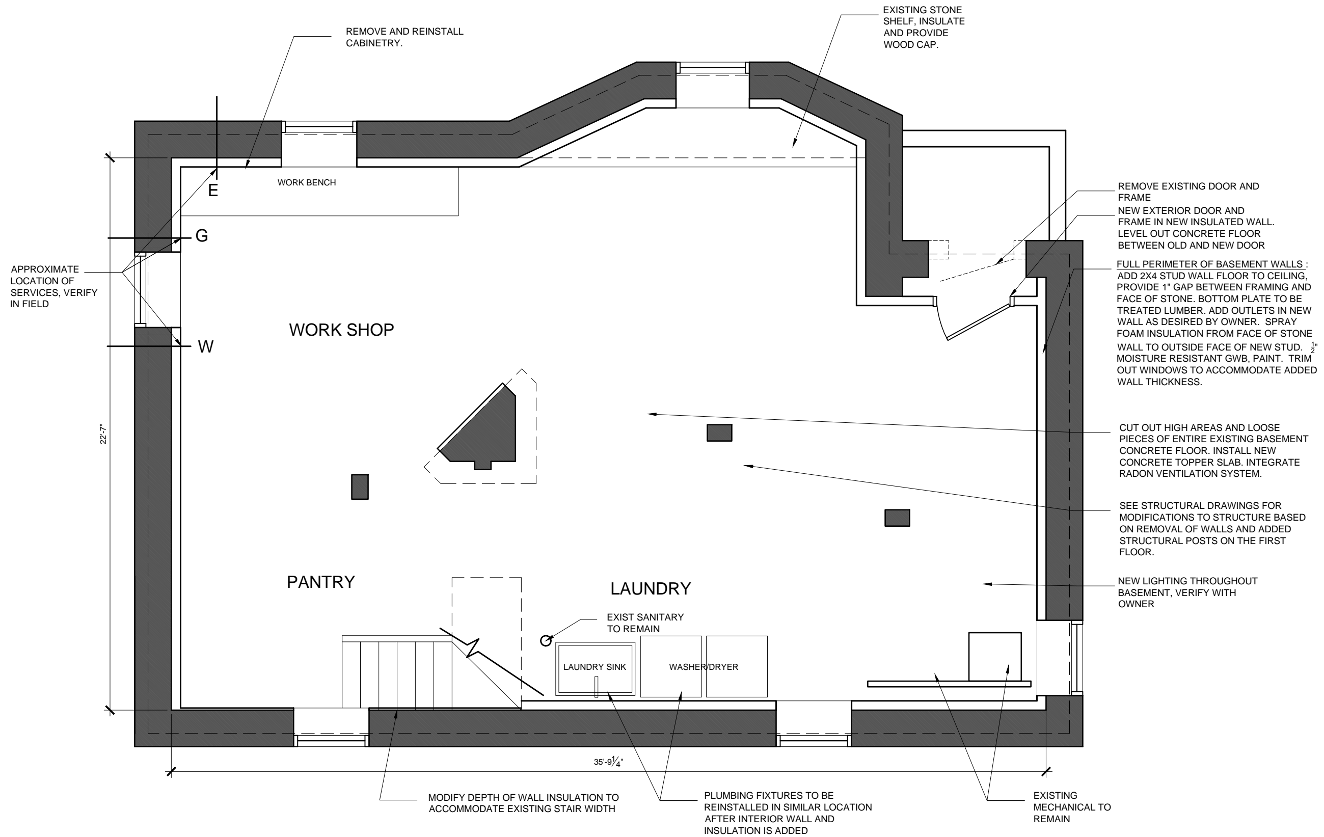
1 BASEMENT PLAN SCALE: 1/4" = 1'-0"
