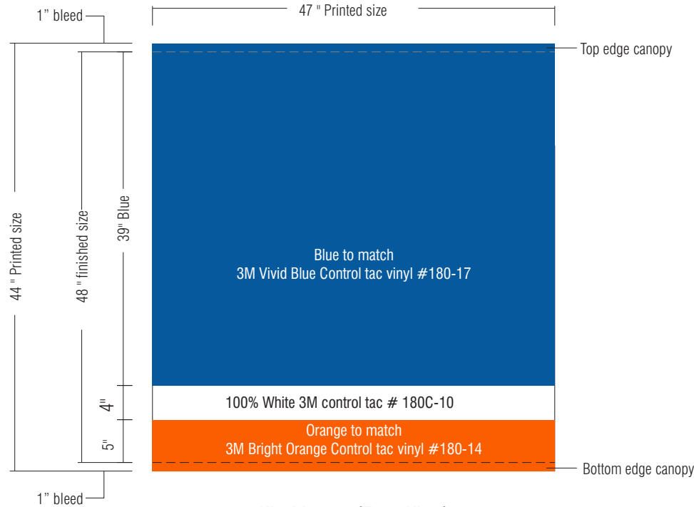
Vinyl Layout (Front View) Scale: 3/4" = 1'-0"
