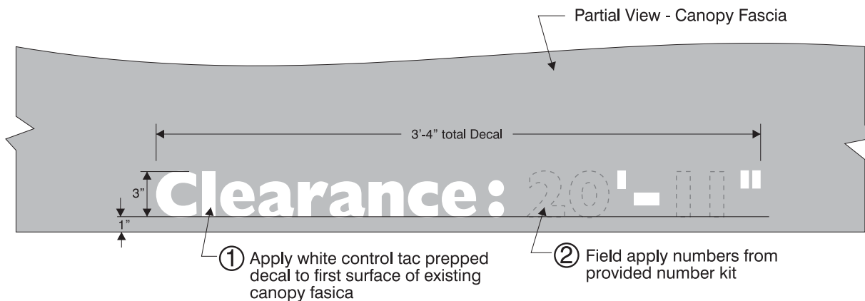
Front View - scale: NTS
