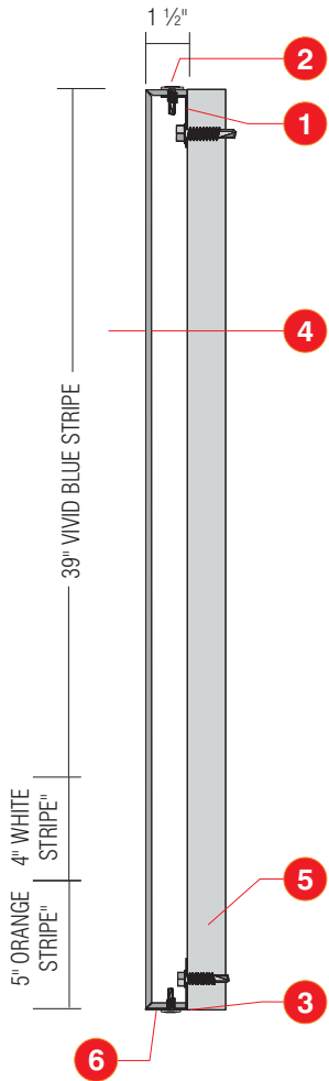
Section Details
