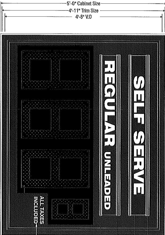
FRONT VIEW SCALE: 3/4" = 1'-0"
