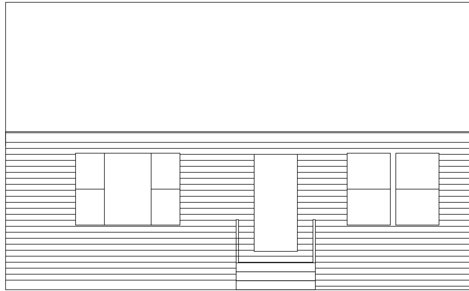
WEST (FRONT) 1/4" = 1'-0"
