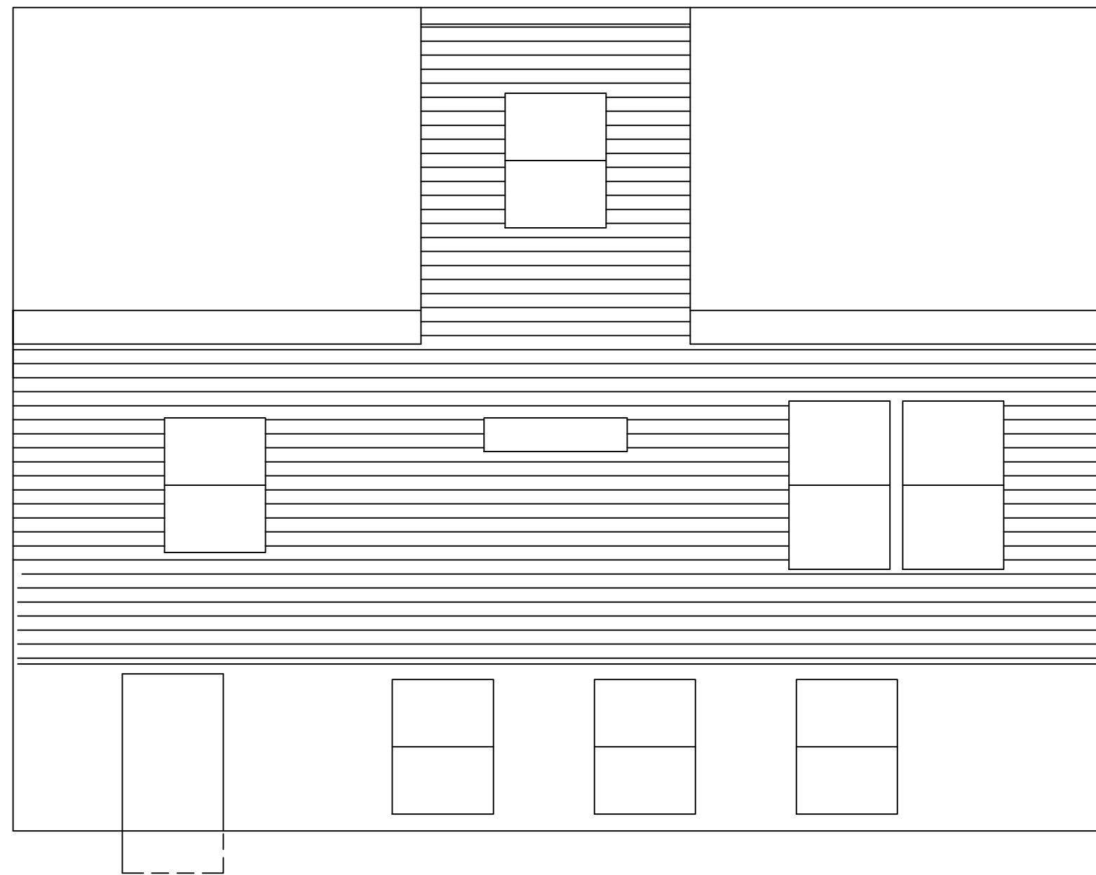
EAST (REAR) 1/4" = 1'-0"
