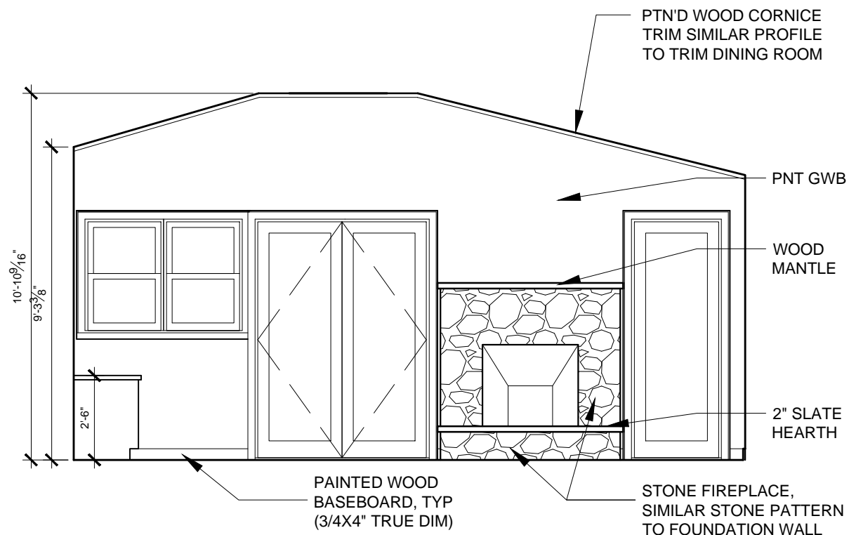
1 GREAT ROOM - WEST ELEVATION SCALE: 1/4" = 1'-0"
