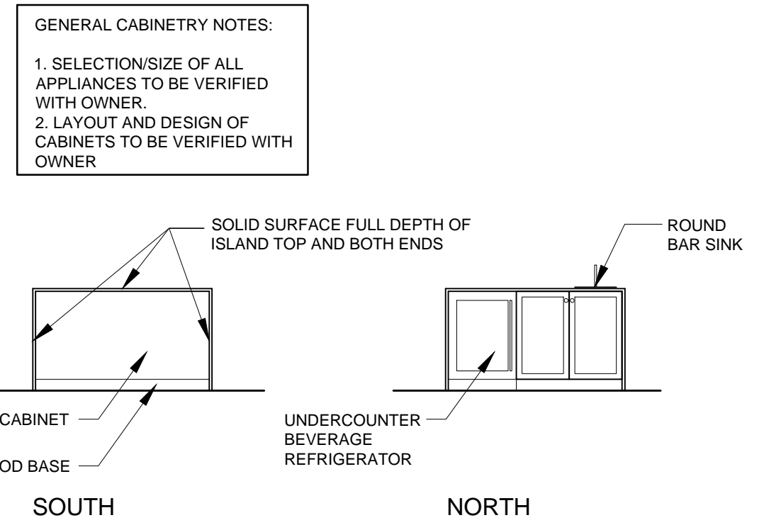
4 ISLAND - NORTH AND SOUTH ELEVATION SCALE: 1/4" = 1'-0"
