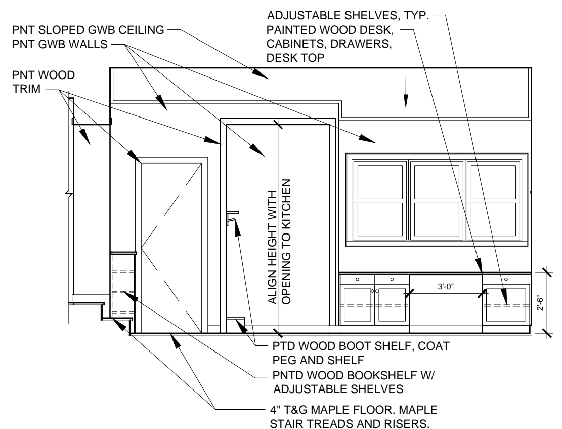
2 GREAT ROOM - SOUTH ELEVATION SCALE: 1/4" = 1'-0"
