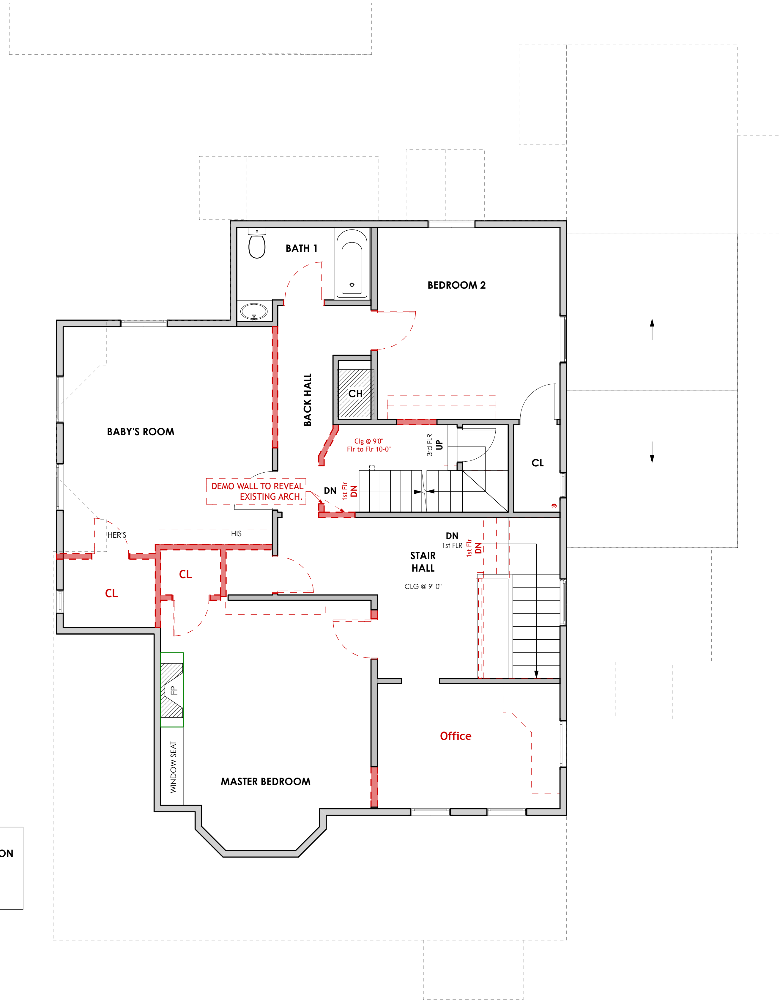
2 SECOND FLOOR DEMOLITION SCALE: 1/4" = 1'-0"
