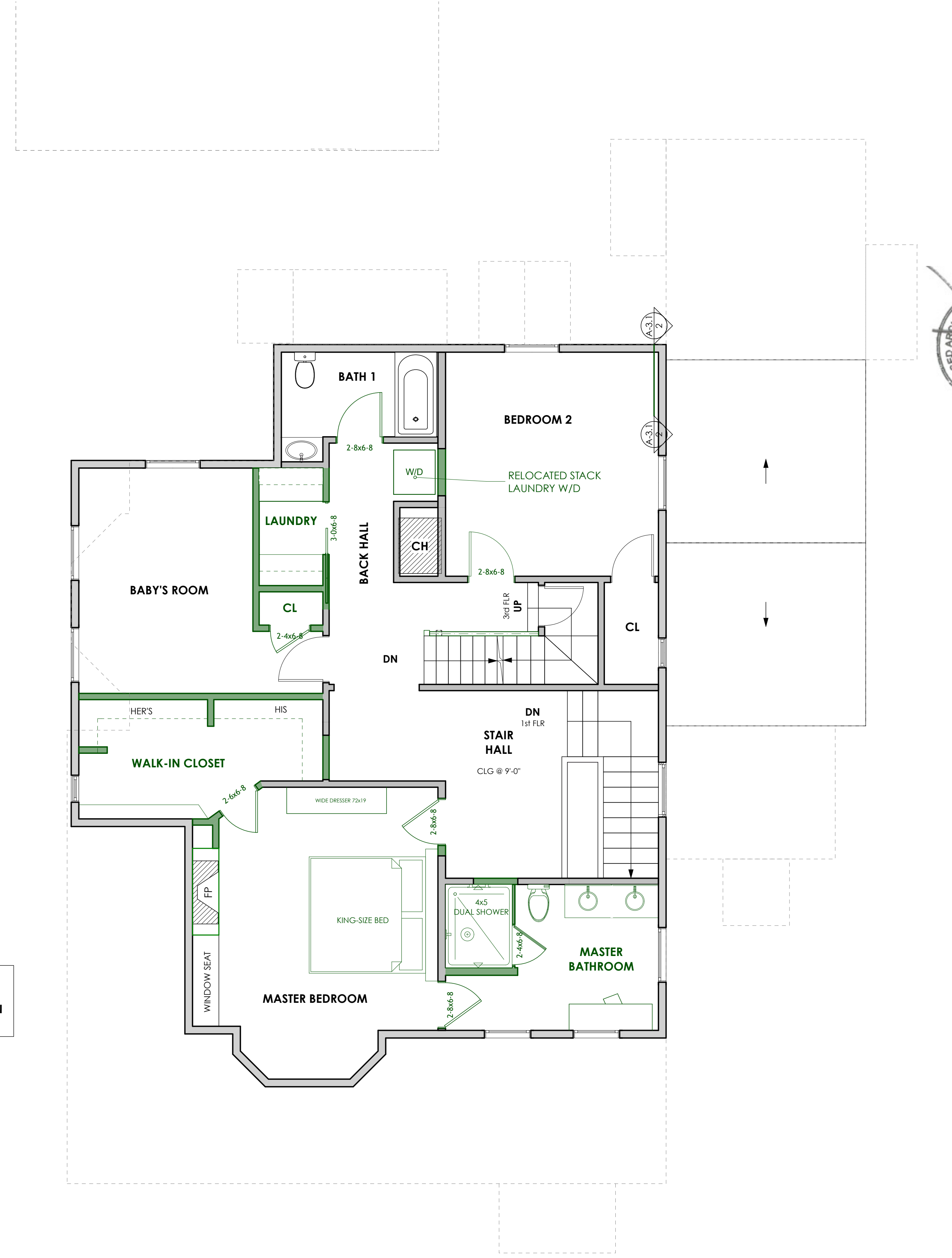
2 PROPOSED SECOND FLOOR SCALE: 1/4" = 1'-0"
