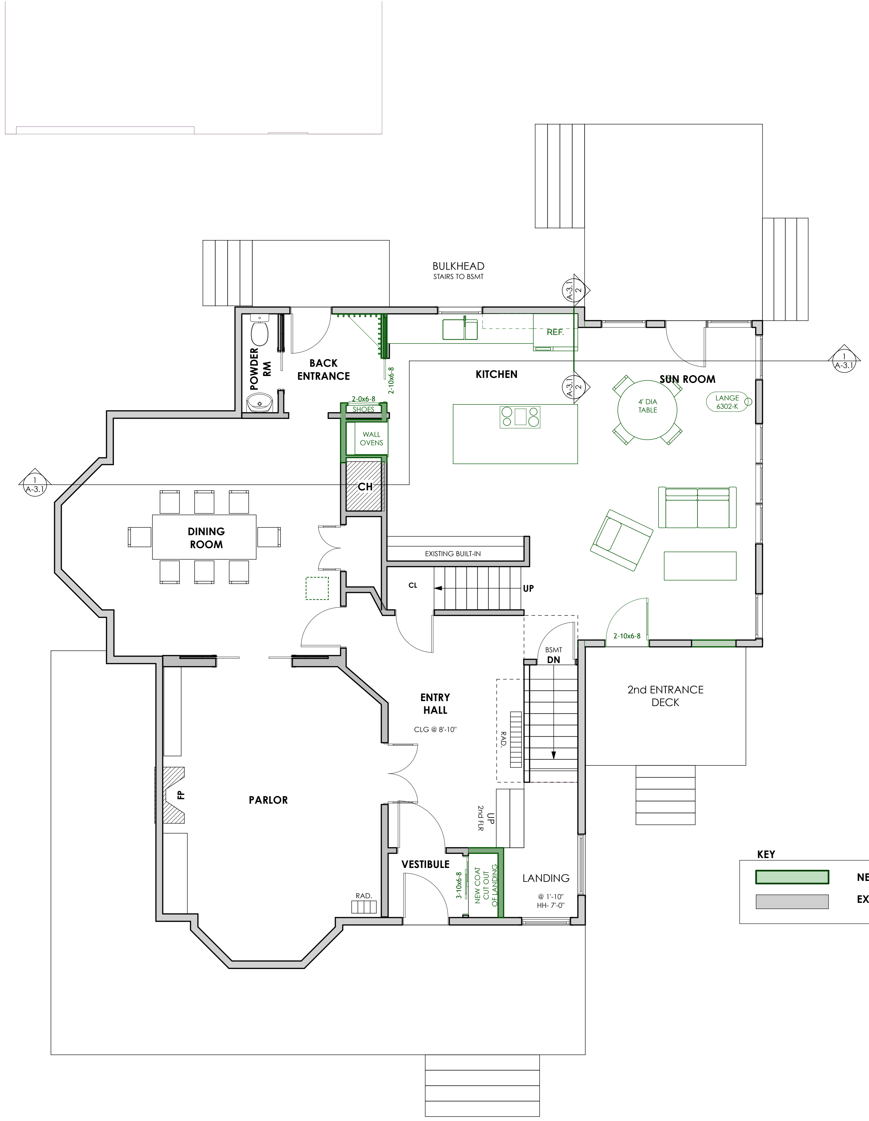
3 1st Flr Plan Proposed SCALE: 1/4" = 1'-0"
