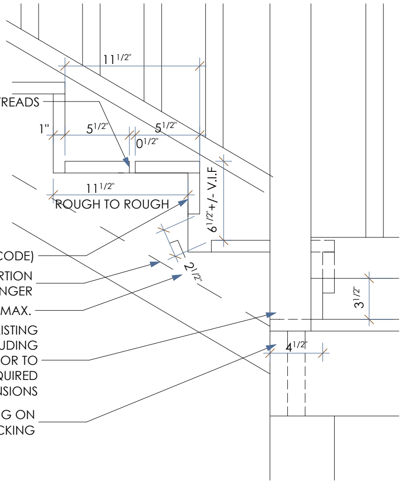
2 ELEVATION DETAIL SCALE: 1 1/2" = 1'-0"
