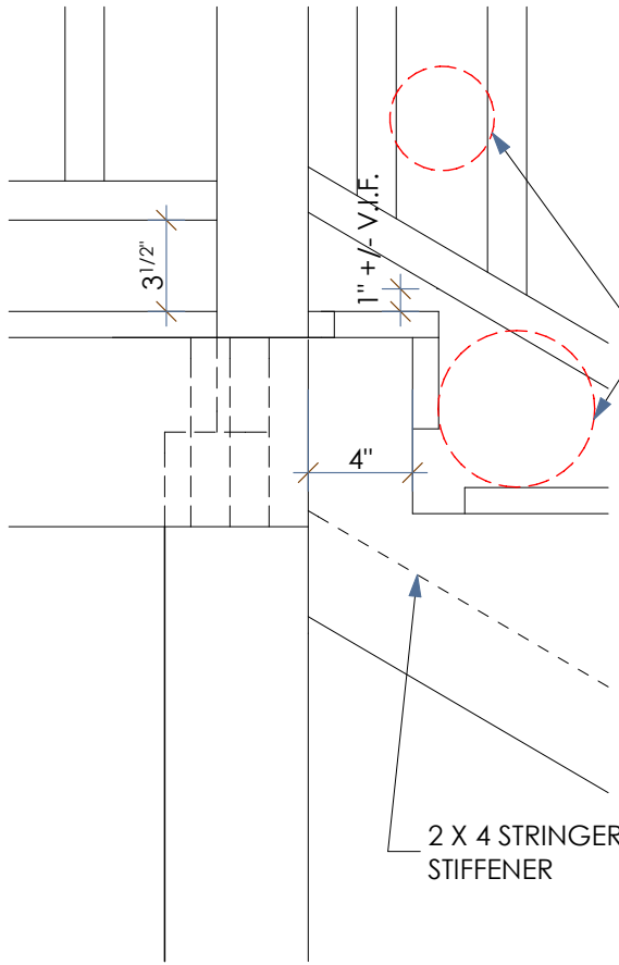
1 ELEVATION DETAIL SCALE: 1 1/2" = 1'-0"
