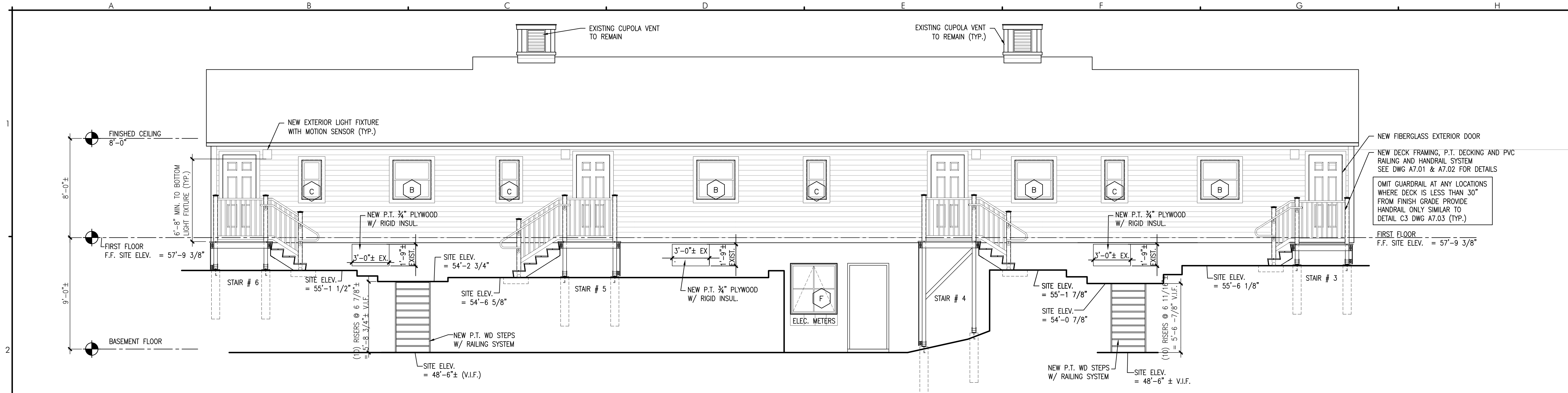
A2 BUILDING ELEVATION
