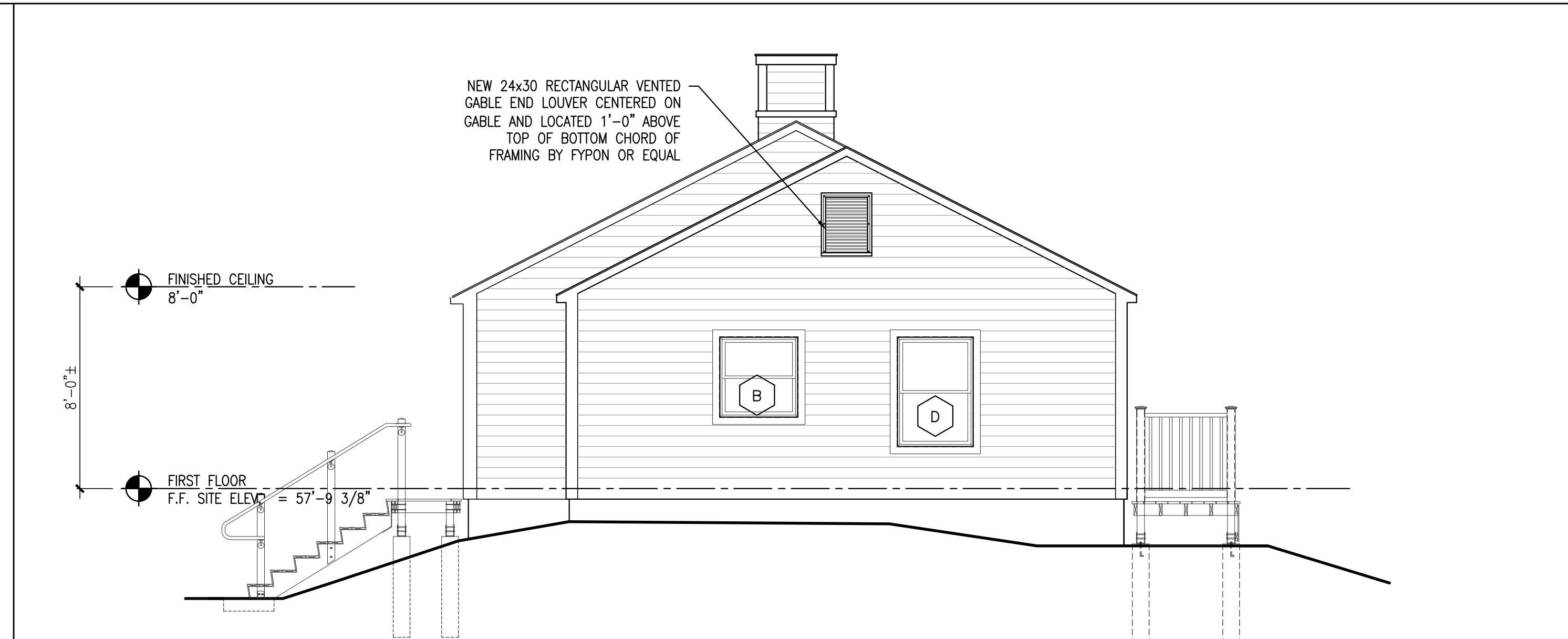
E5 BUILDING ELEVATION
