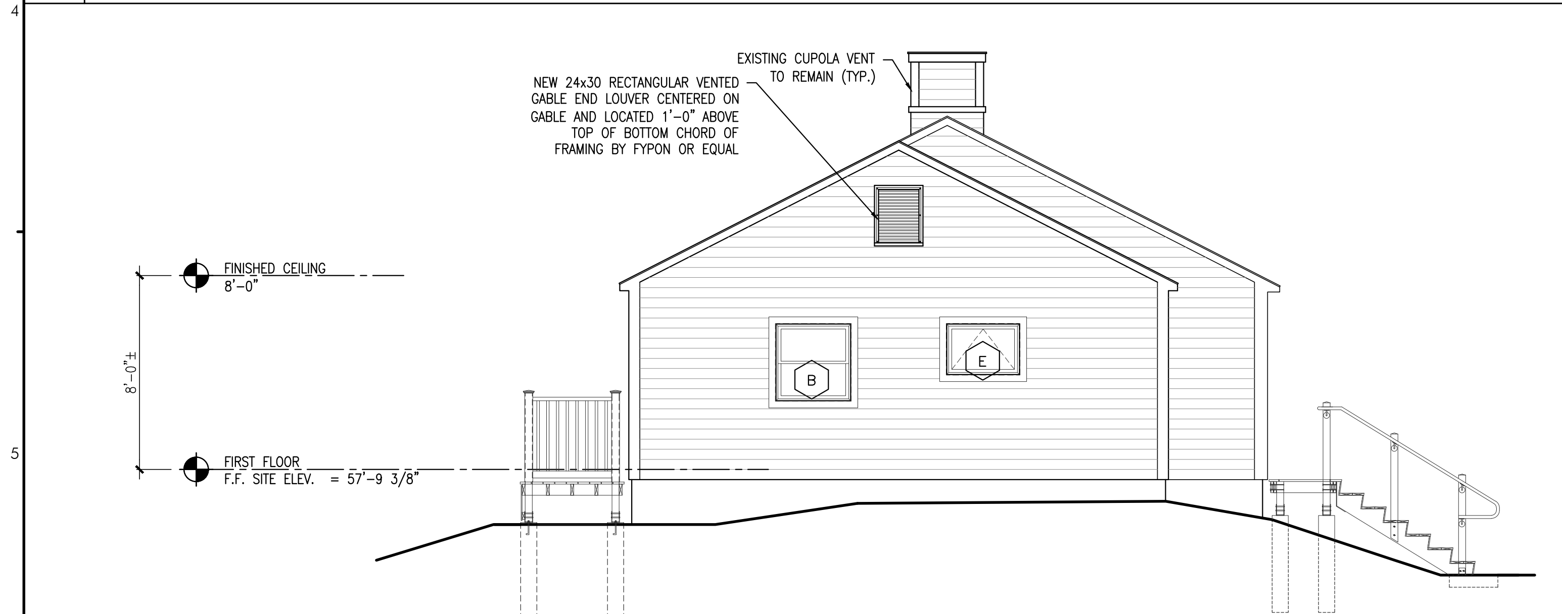
A5 BUILDING ELEVATION
