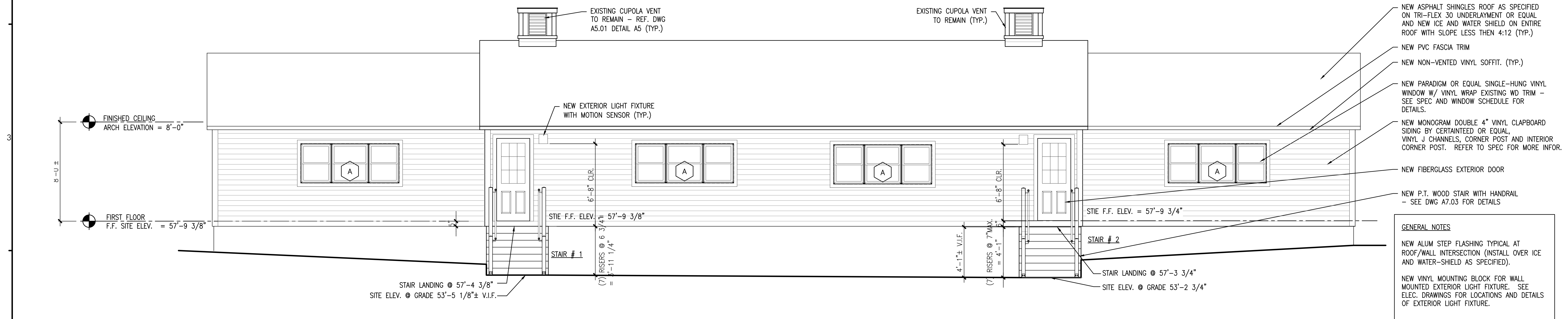
A4 BUILDING ELEVATION
