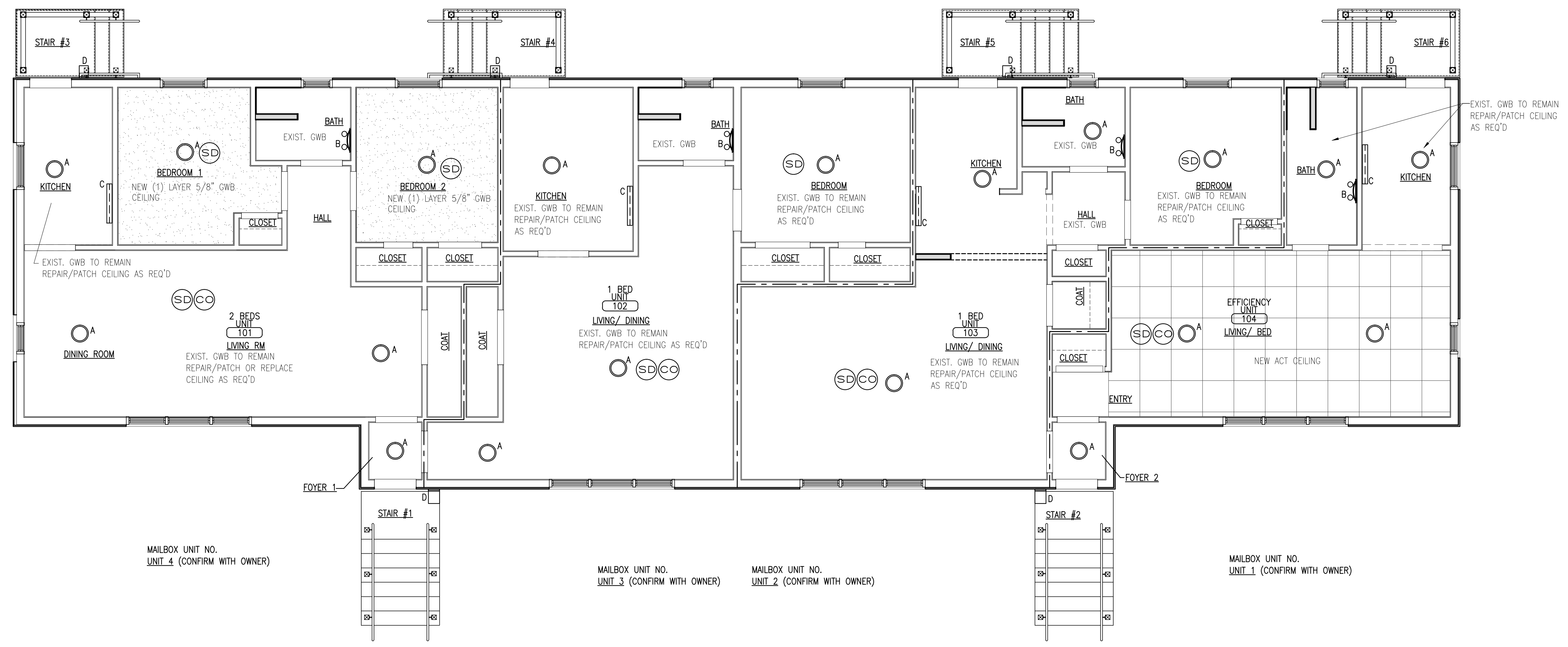
A3 FIRST FLOOR REFLECTED CEILING PLAN REFERENCED FROM: SCALE: 1/4" = 1'-0"
