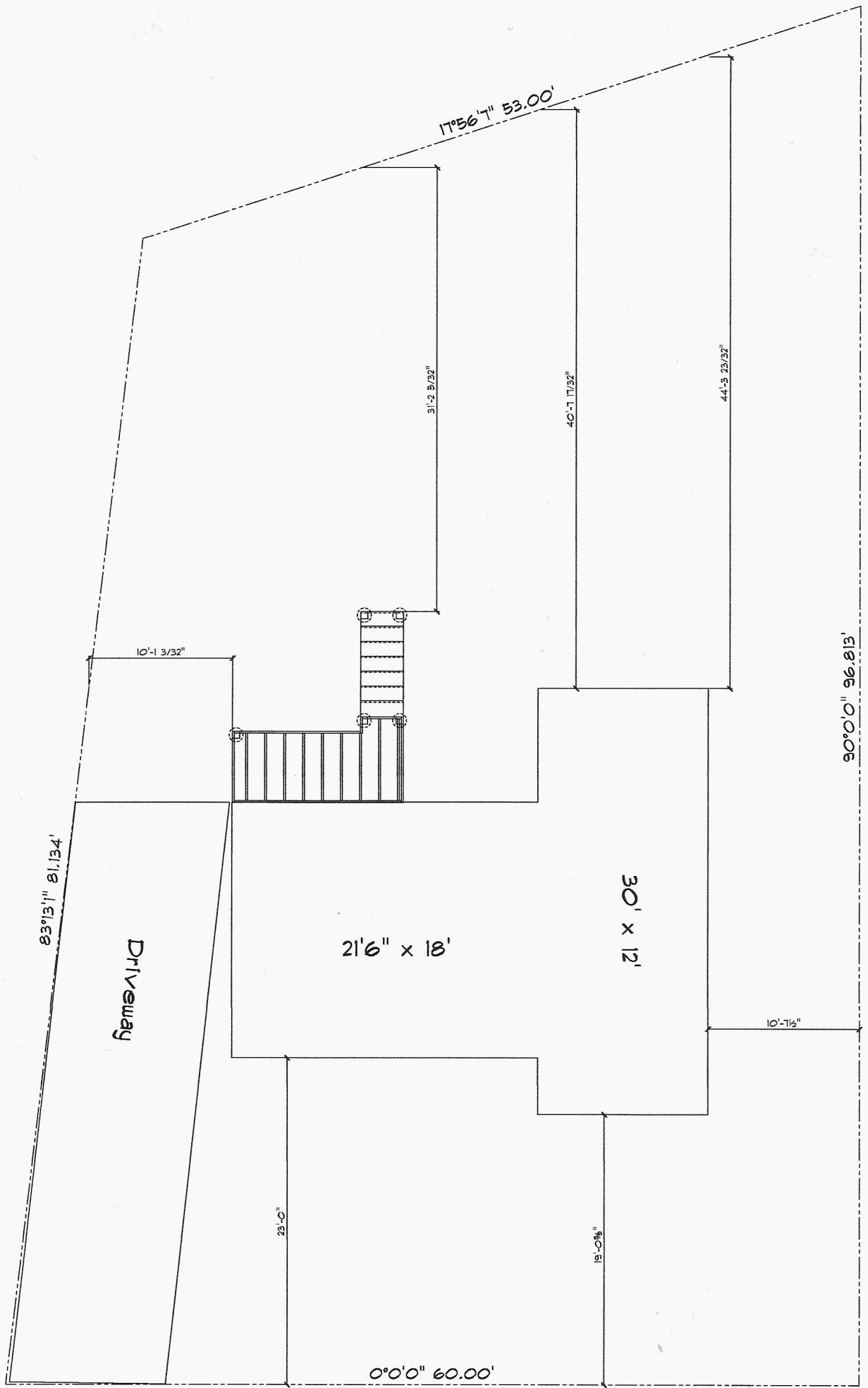
Site Plan
