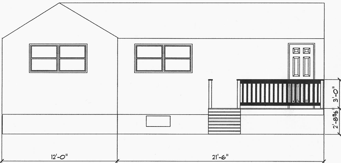
East Elevation Proposed Deck
