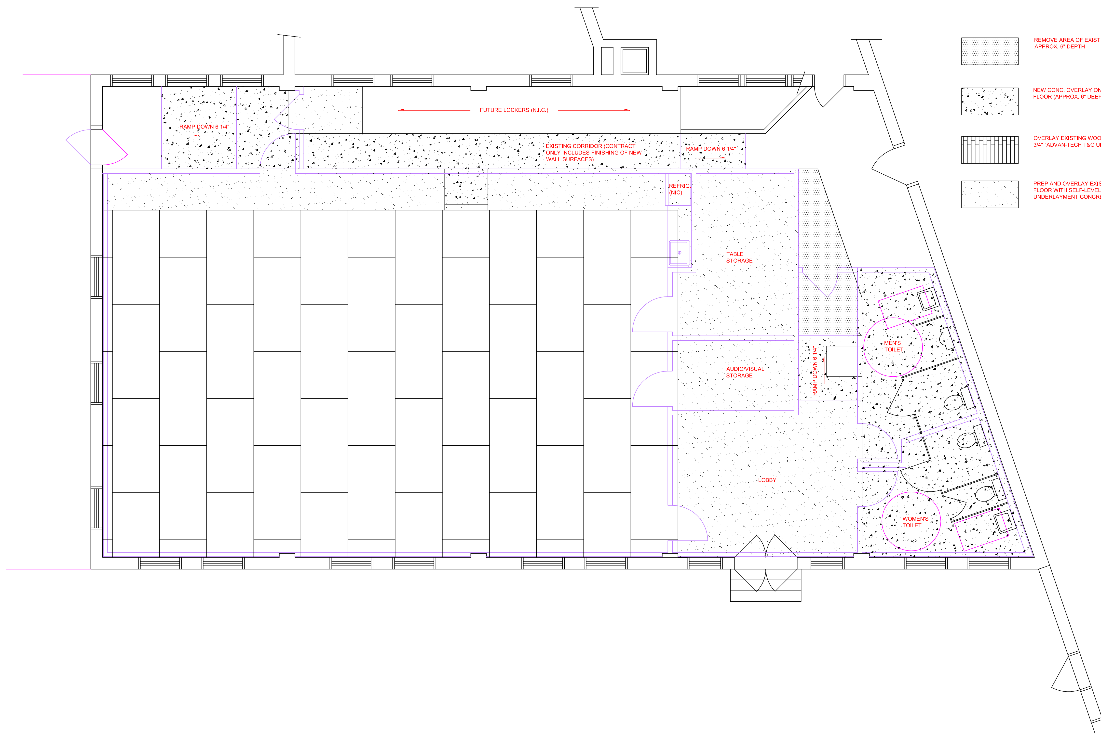
PROPOSED UNDERLAYMENT AND FLOOR PREP AT METER SHOP
