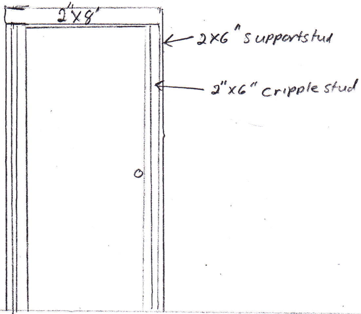
Header Detail going from mudroom to existing House
