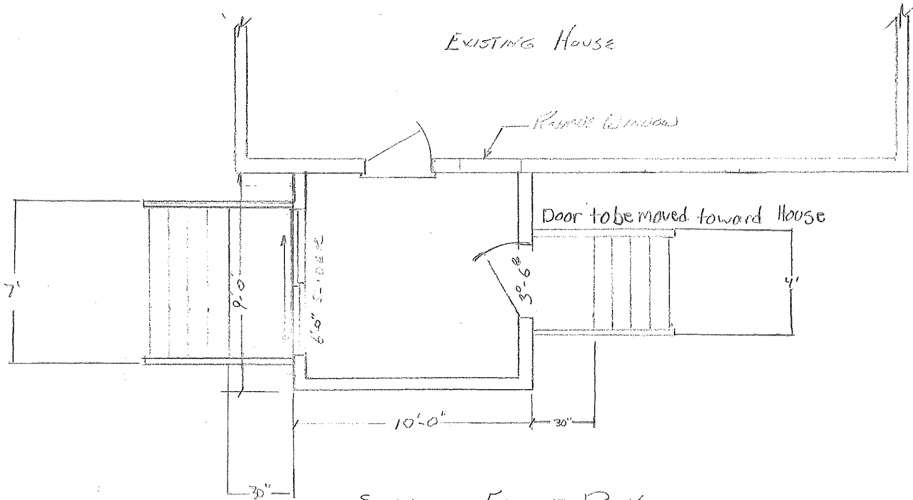
SIDE FLOOR PLAN
