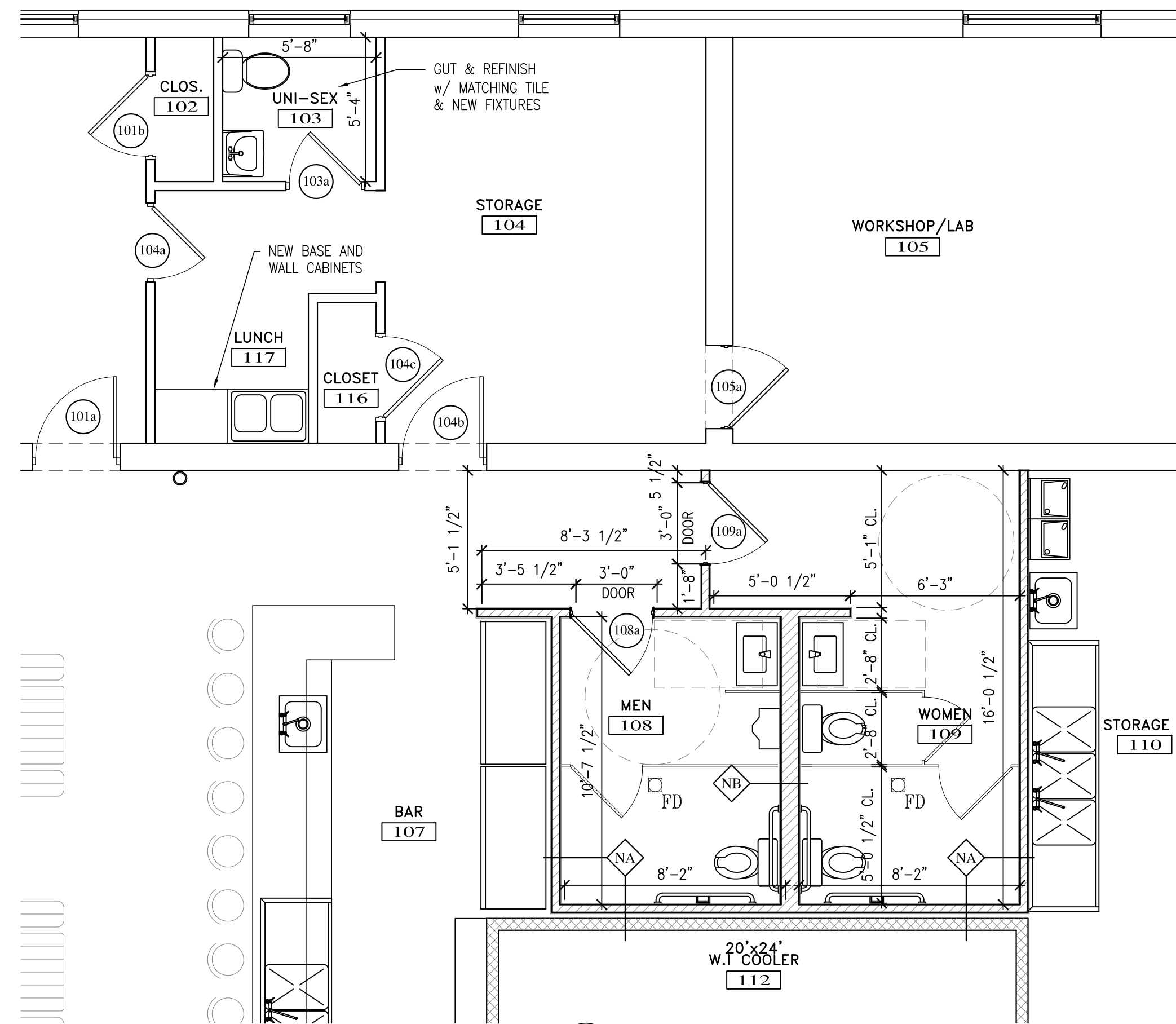
1 ENLARGED PLAN A1.1 SCALE: 1/4" = 1'-0"
