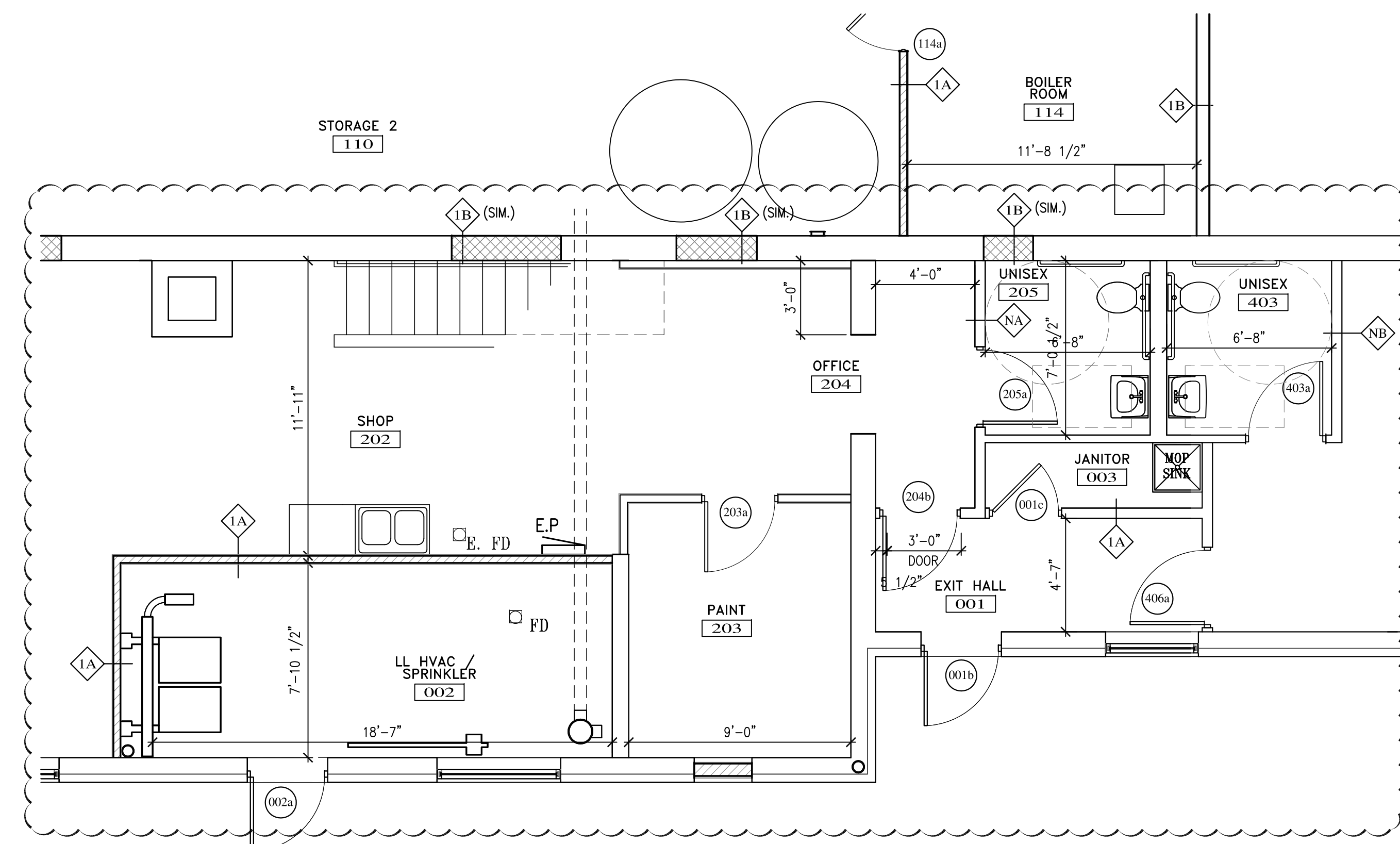
3 ENLARGED PLAN A1.1 SCALE: 1/4" = 1'-0"
