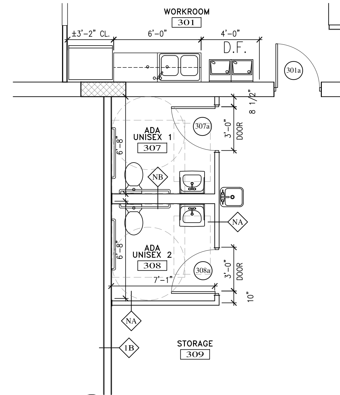
2 ENLARGED PLAN A1.1 SCALE: 1/4" = 1'-0"
