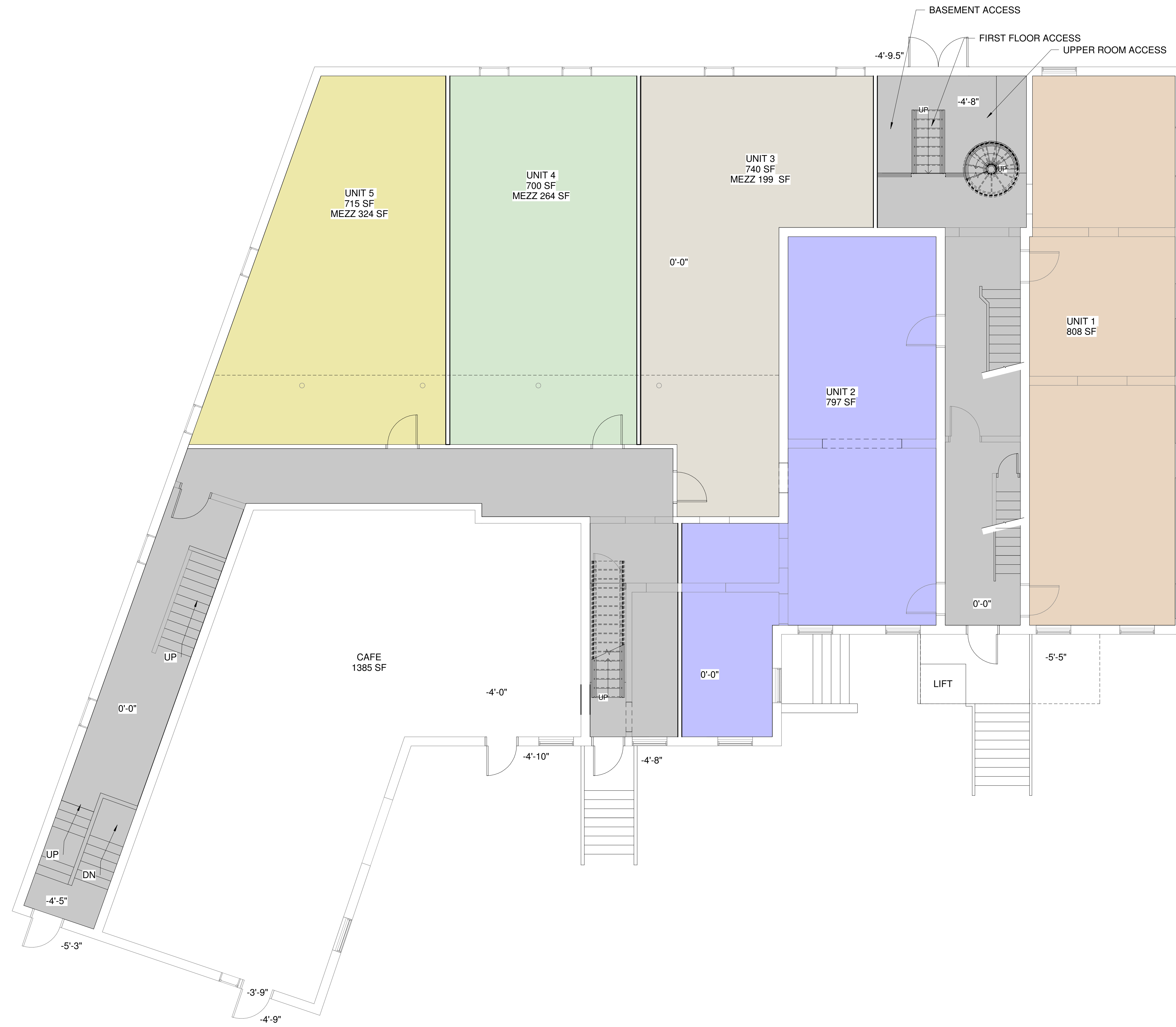
1 FIRST FLOOR 3/16" = 1'-0"
