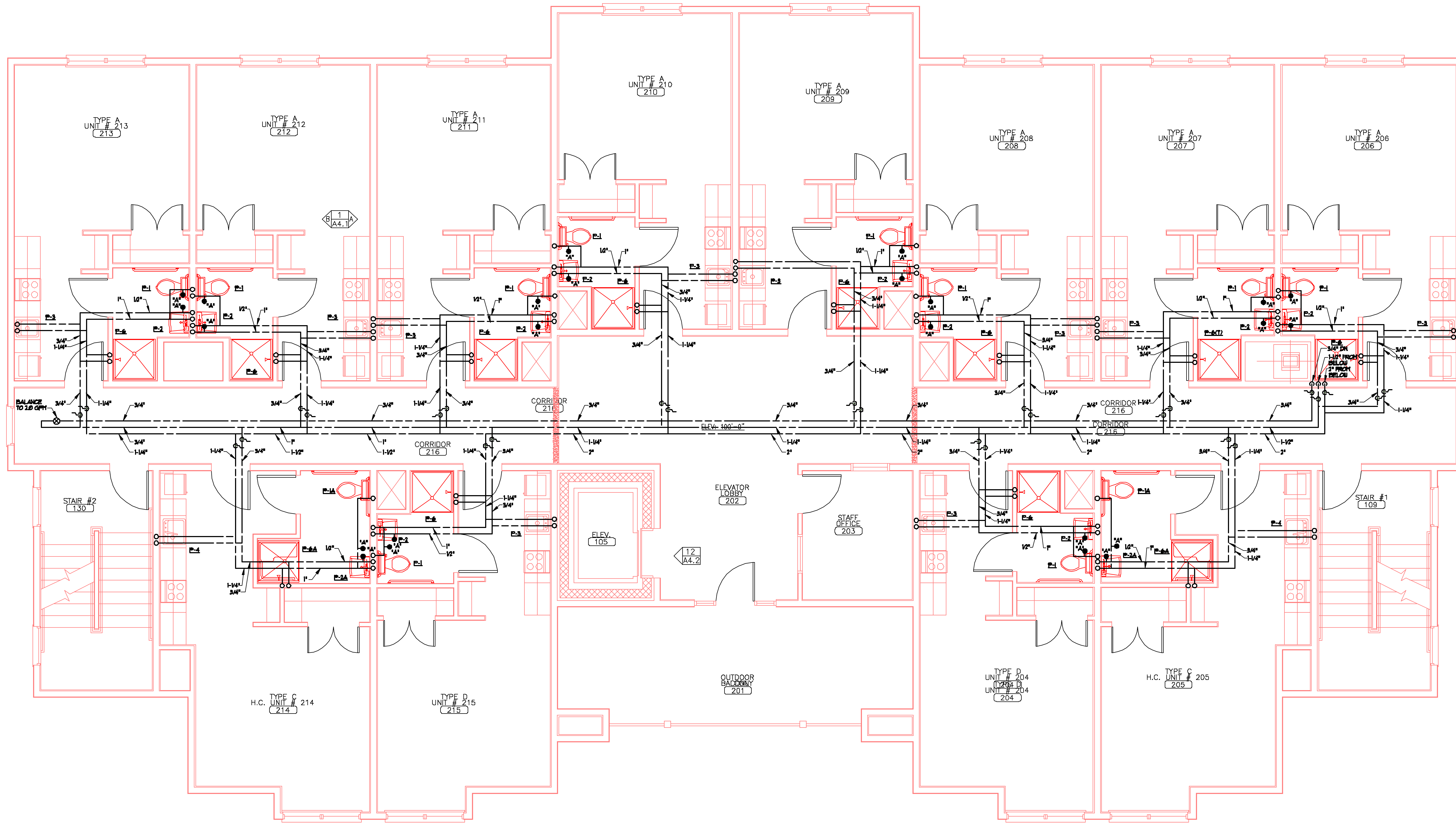
SECOND FLOOR DOMESTIC PLUMBING PLAN SCALE 1/4" = 1'-0"
