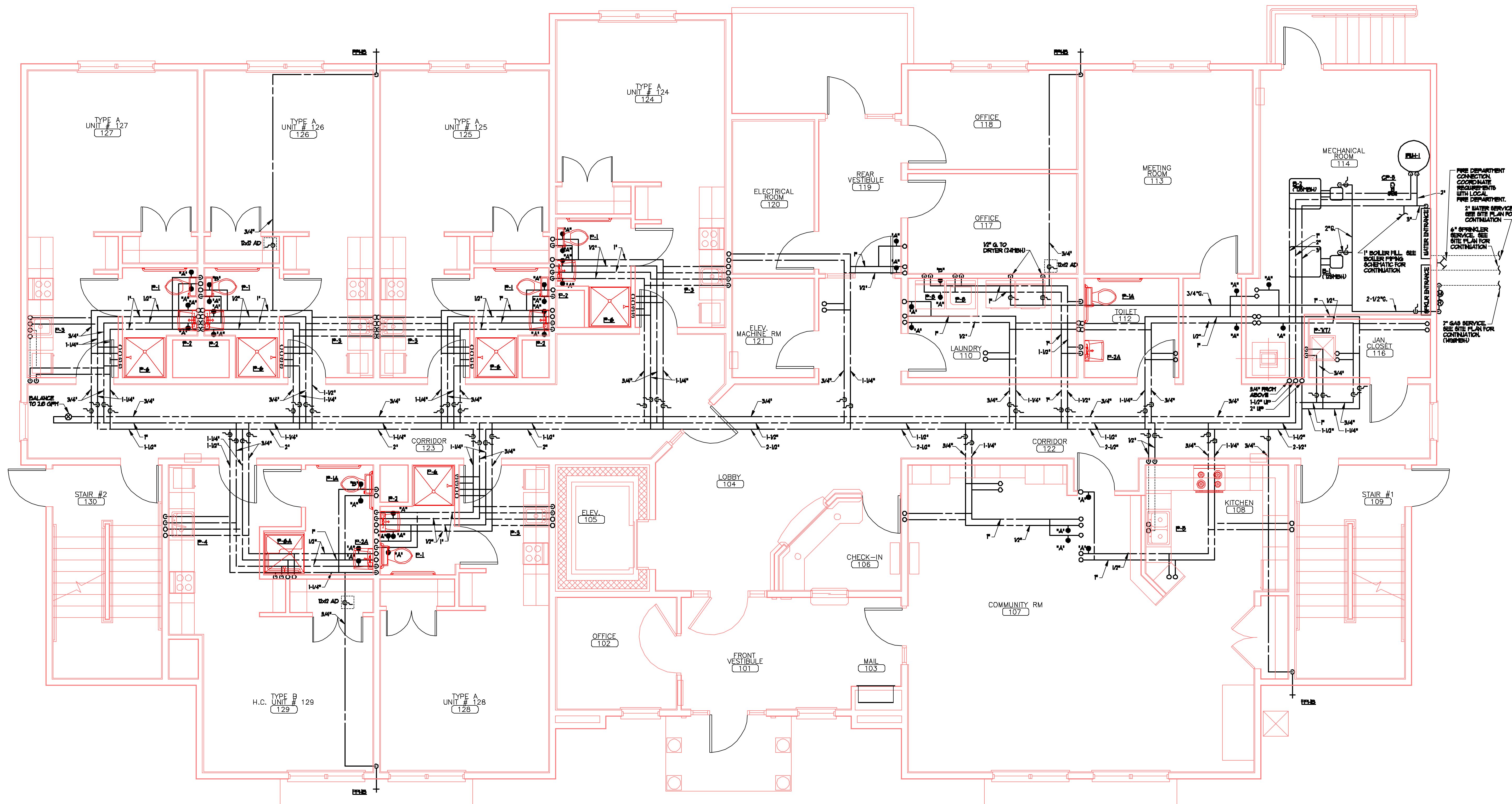
FIRST FLOOR DOMESTIC PLUMBING PLAN SCALE 1/4" = 1'-0"
