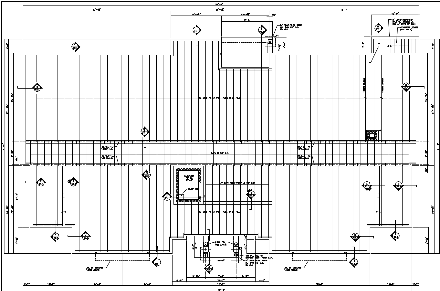
FIRST FLOOR FRAMING PLAN 1/4" = 1'-0"
