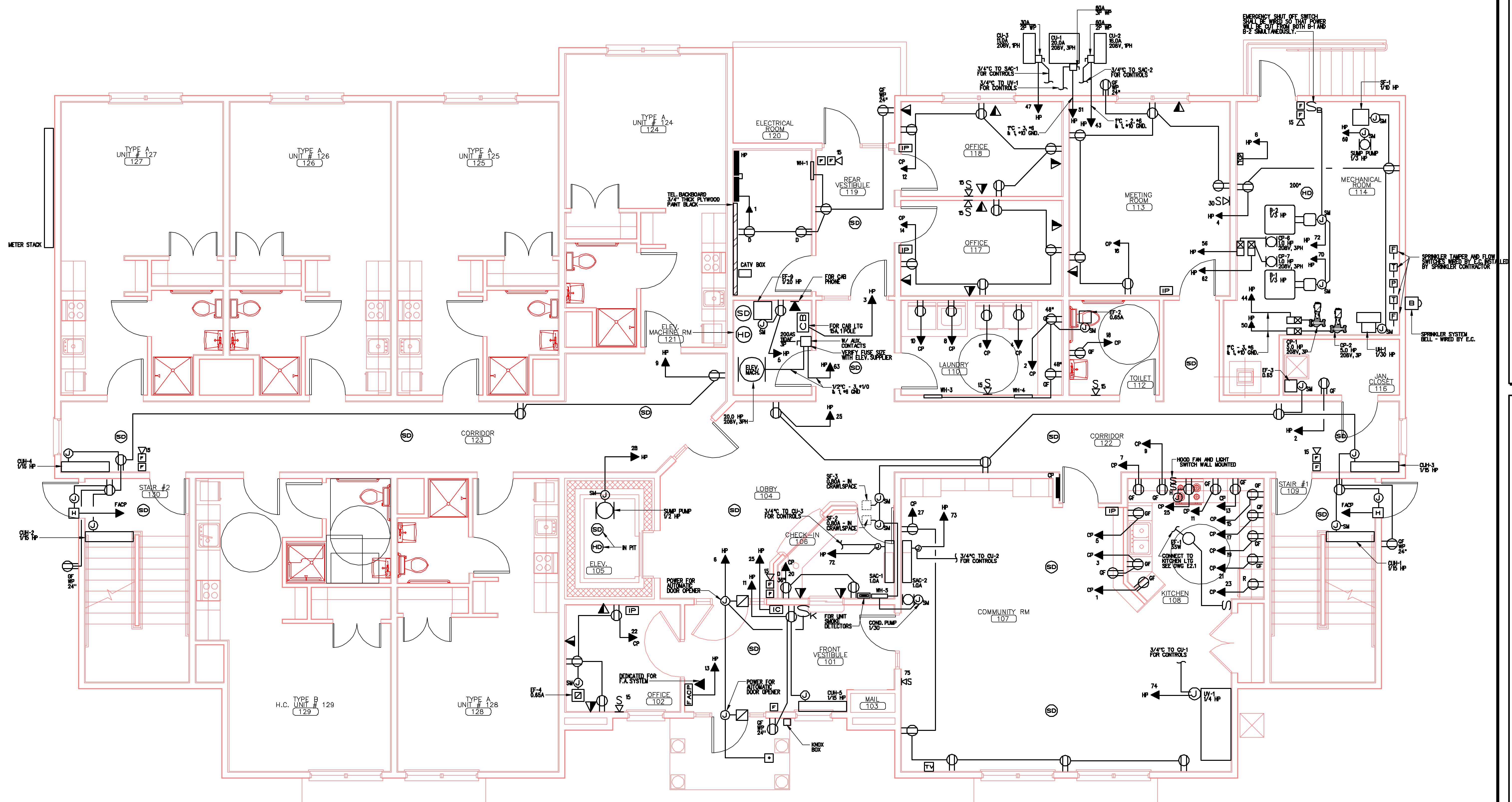
FIRST FLOOR POWER PLAN SCALE: 1/4"=1'-0"
