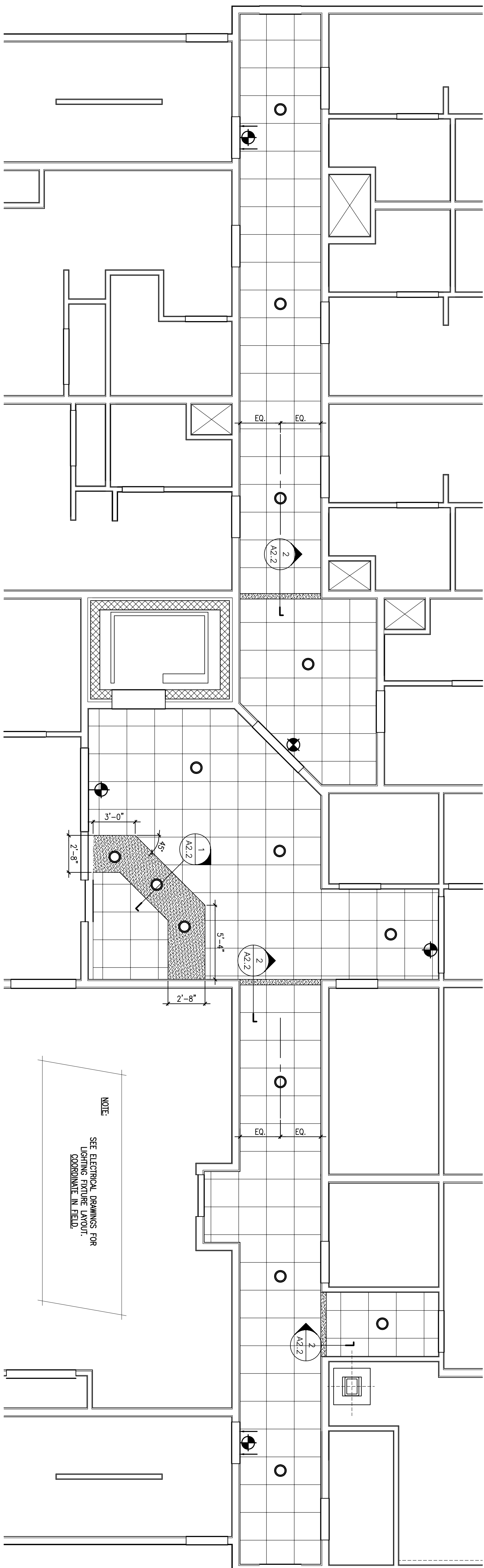
FIRST FLOOR REFLECTED CEILING PLAN SCALE: 1/4" = 1'-0"
