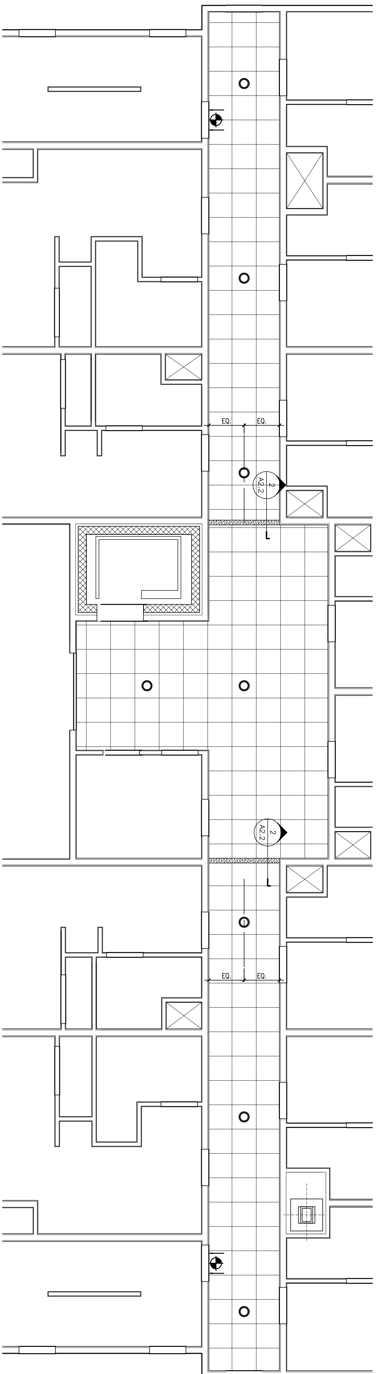
SECOND FLOOR REFLECTED CEILING PLAN SCALE: 1/4" = 1'-0"
