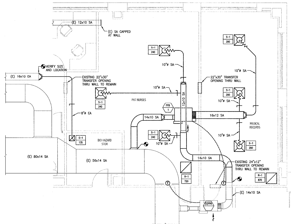
1 HVAC PLAN 1/4" = 1'-0"
