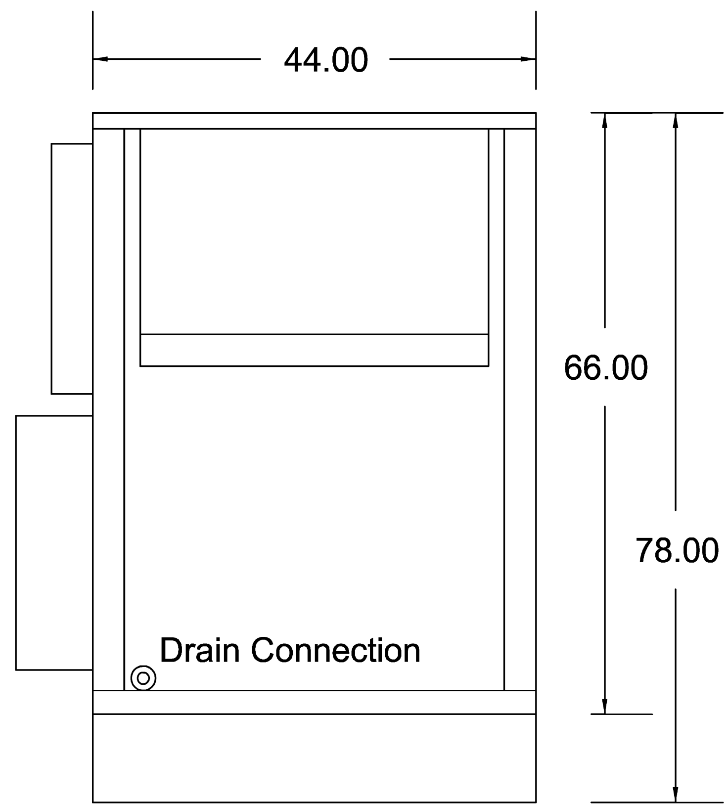
Right End ( elev. view )
