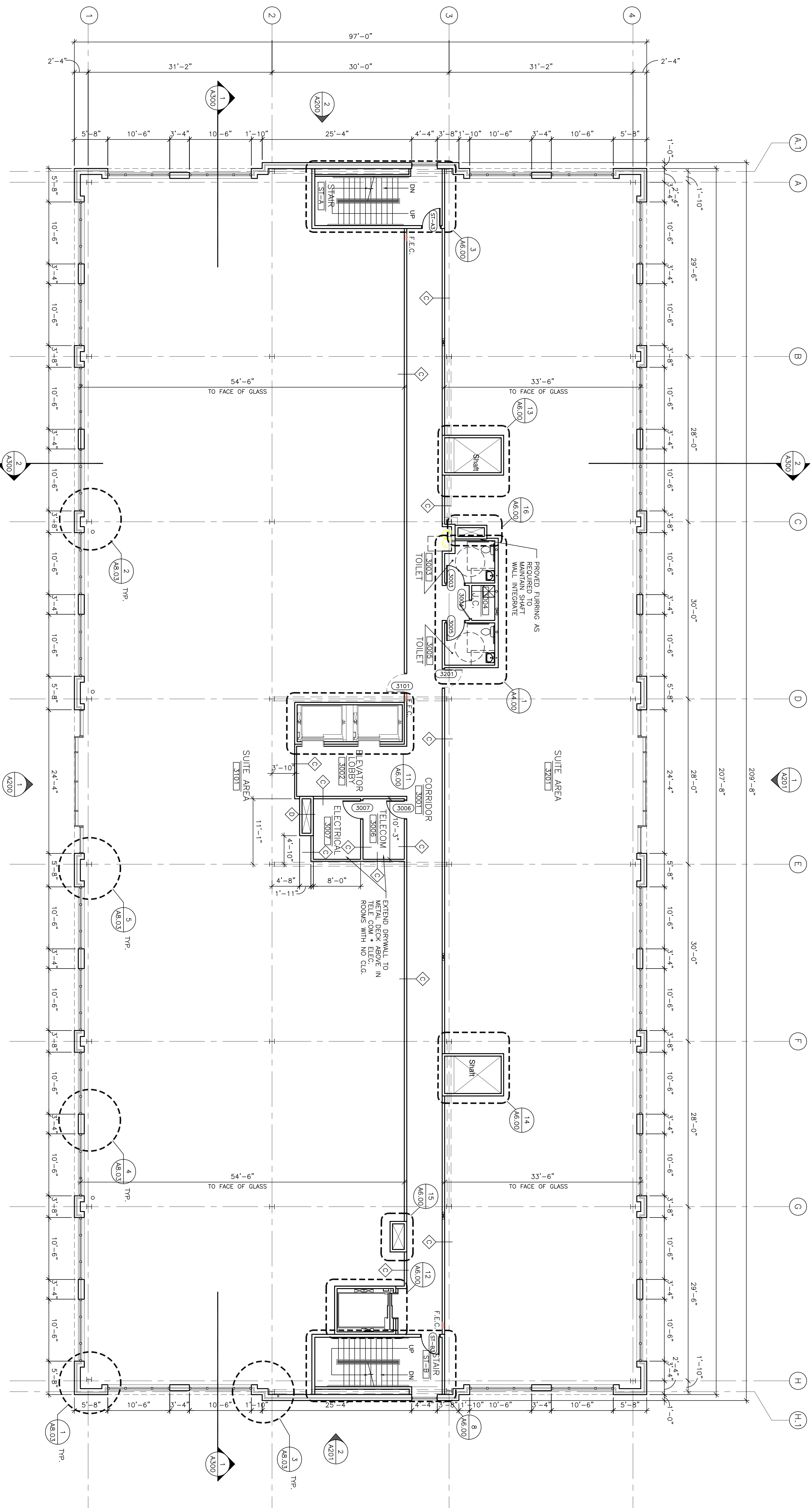
1 THIRD FLOOR CONSTRUCTION PLAN 1/8"=1'-0"
