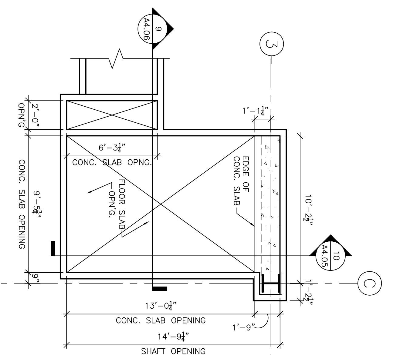
4 THIRD FLOOR NORTH SHAFT SCALE: 1/4\"/>
