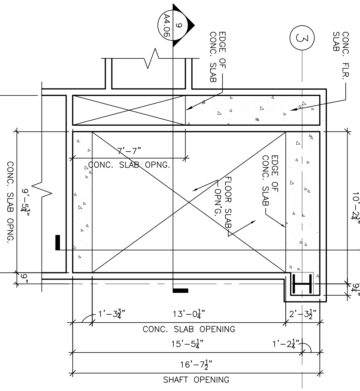
5 FOURTH FLOOR NORTH SHAFT SCALE: 1/4\"/>
