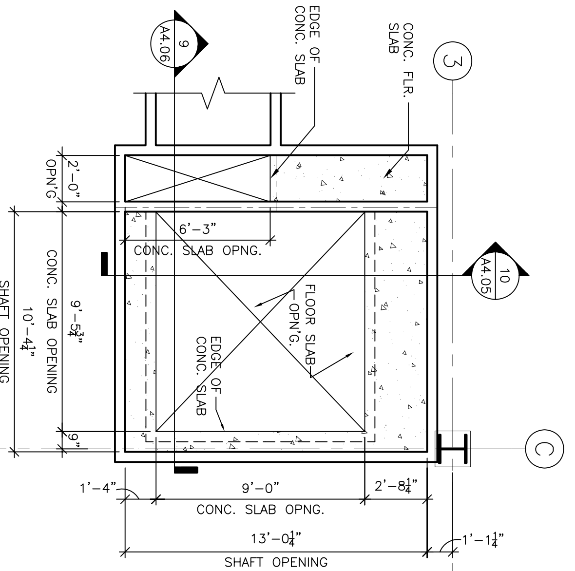
3 SECOND FLOOR NORTH SHAFT SCALE: 1/4\"/>
