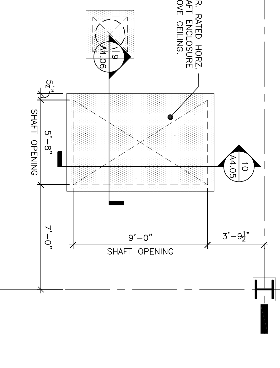
1 GROUND FLOOR NORTH SHAFT ABOVE CEILING SCALE: 1/4\"/>
