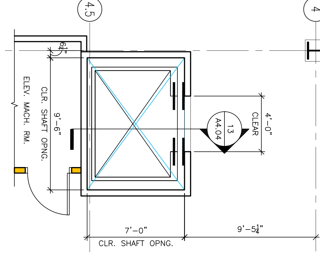
2 SOILED ELEVATOR #5 GROUND FLOOR SCALE: 1/4"=1'-0"
