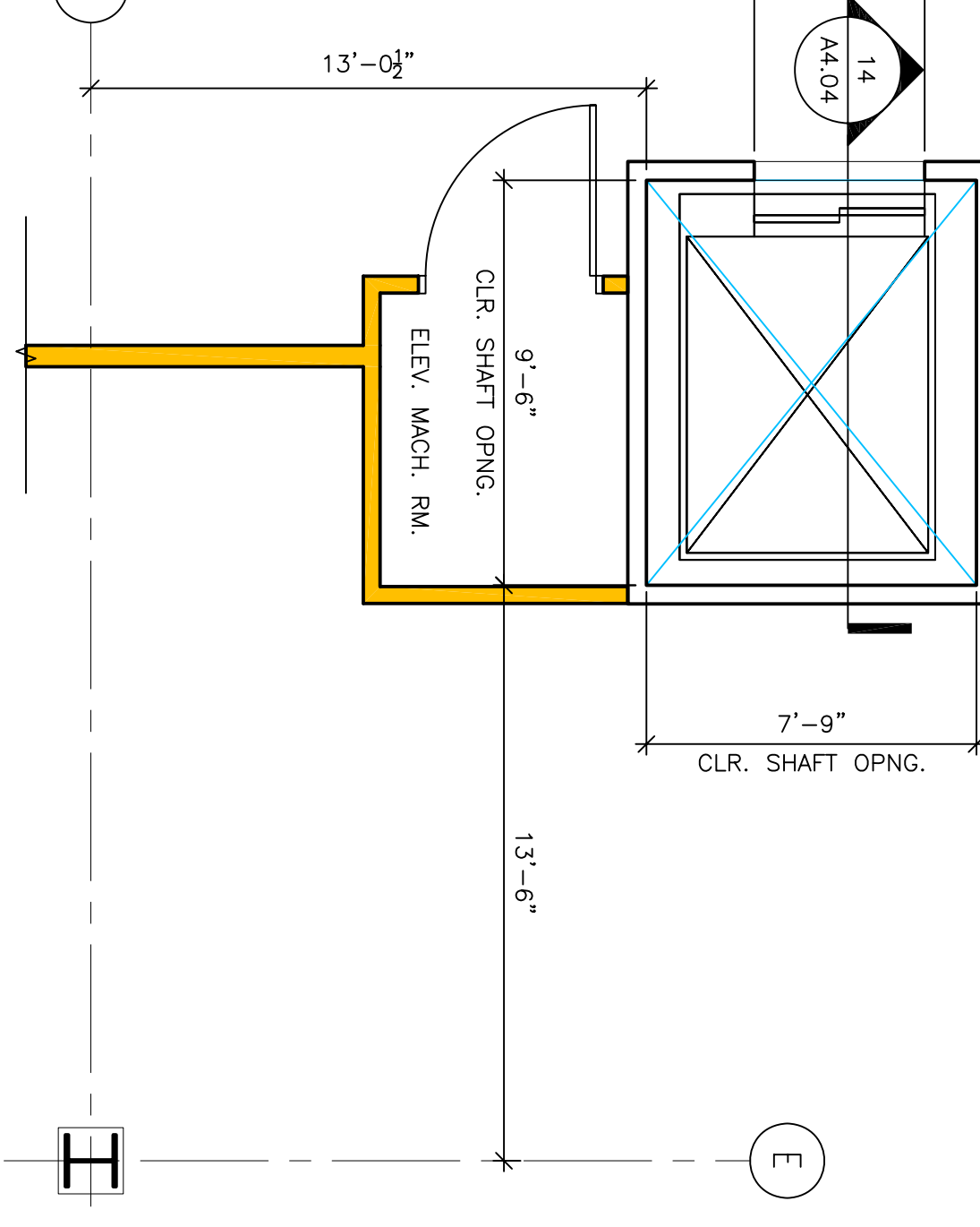
6 CLEAN ELEVATOR #6 GROUND FLOOR SCALE: 1/4"=1'-0"
