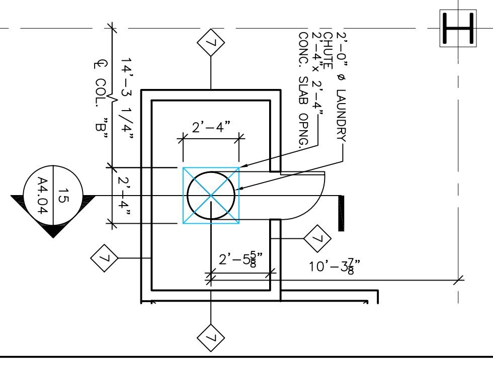
9 LAUNDRY CHUTE FIRST FLOOR SCALE: 1/4"=1'-0"
