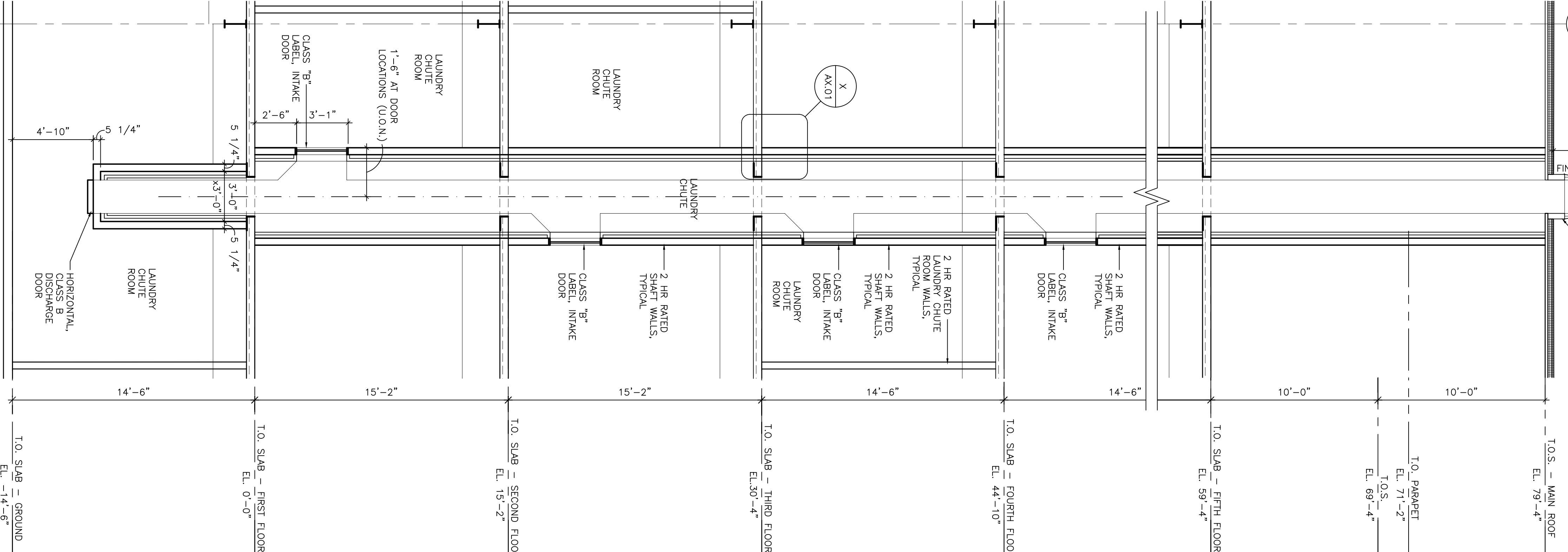
15 LAUNDRY CHUTE SECTION SCALE: 1/4"=1'-0"
