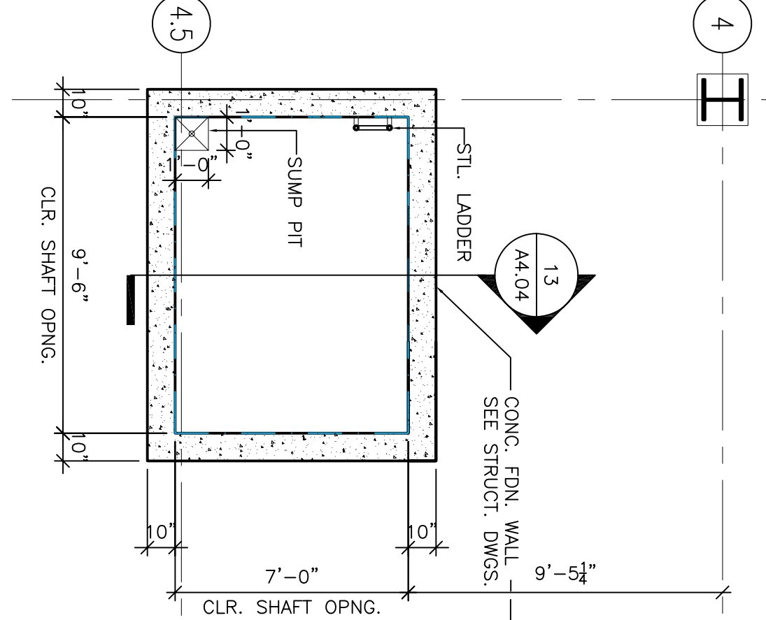
1 SOILED ELEVATOR #5 GROUND FLOOR PIT SCALE: 1/4"=1'-0"
