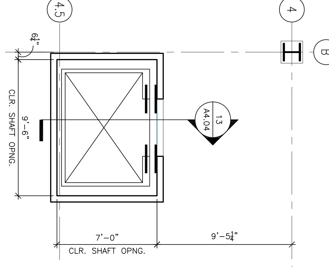
4 SOILED ELEVATOR #5 SECOND FLOOR SCALE: 1/4"=1'-0"
