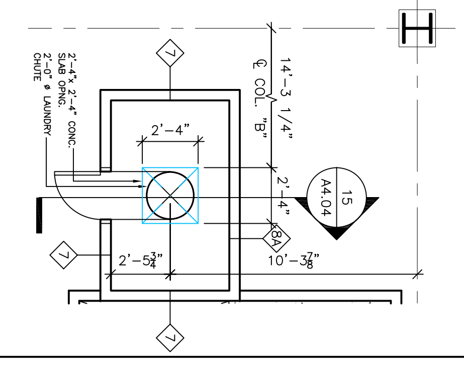
10 LAUNDRY CHUTE SECOND FLOOR SCALE: 1/4"=1'-0"
