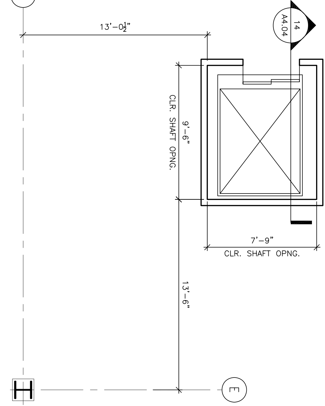
8 CLEAN ELEVATOR #6 SECOND FLOOR SCALE: 1/4"=1'-0"
