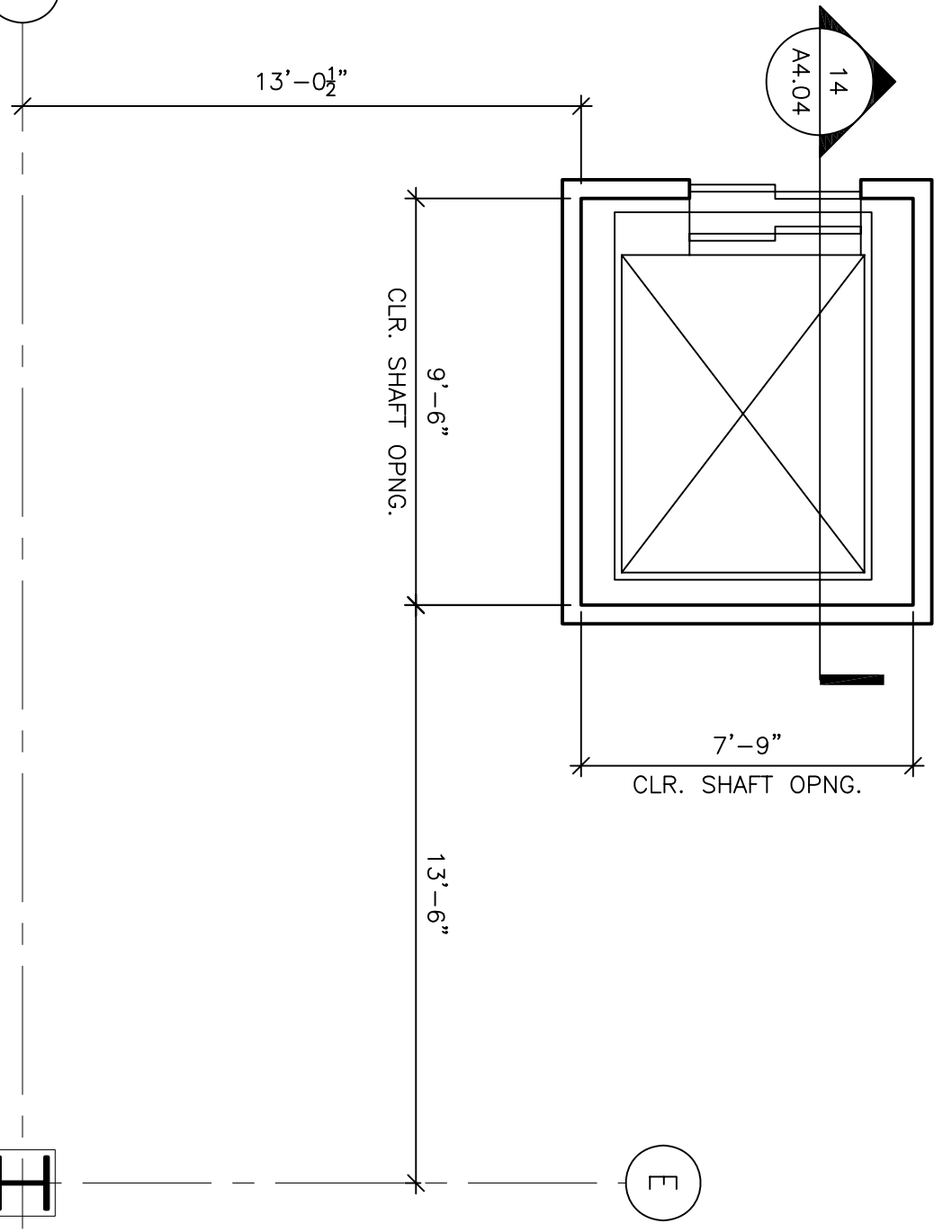
7 CLEAN ELEVATOR #6 FIRST FLOOR SCALE: 1/4"=1'-0"
