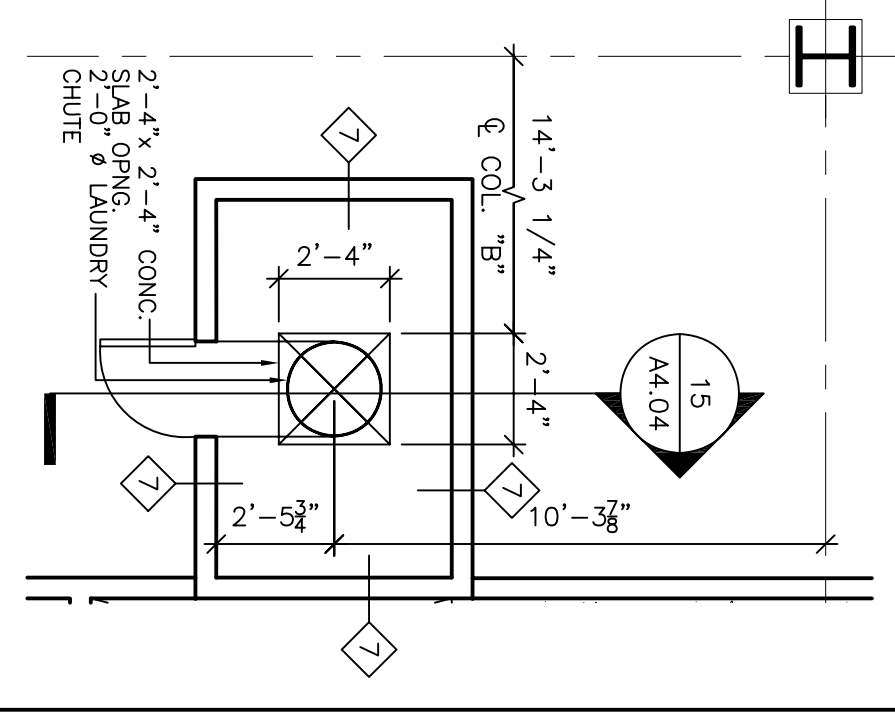
12 LAUNDRY CHUTE FOURTH FLOOR SCALE: 1/4"=1'-0"
