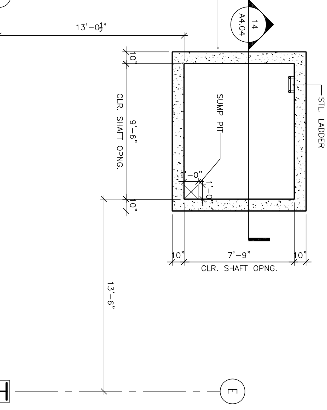
5 CLEAN ELEVATOR #6 GROUND FLOOR PIT SCALE: 1/4"=1'-0"
