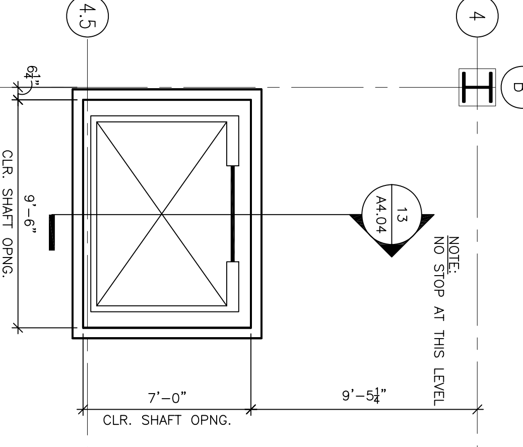
3 SOILED ELEVATOR #5 FIRST FLOOR SCALE: 1/4"=1'-0"
