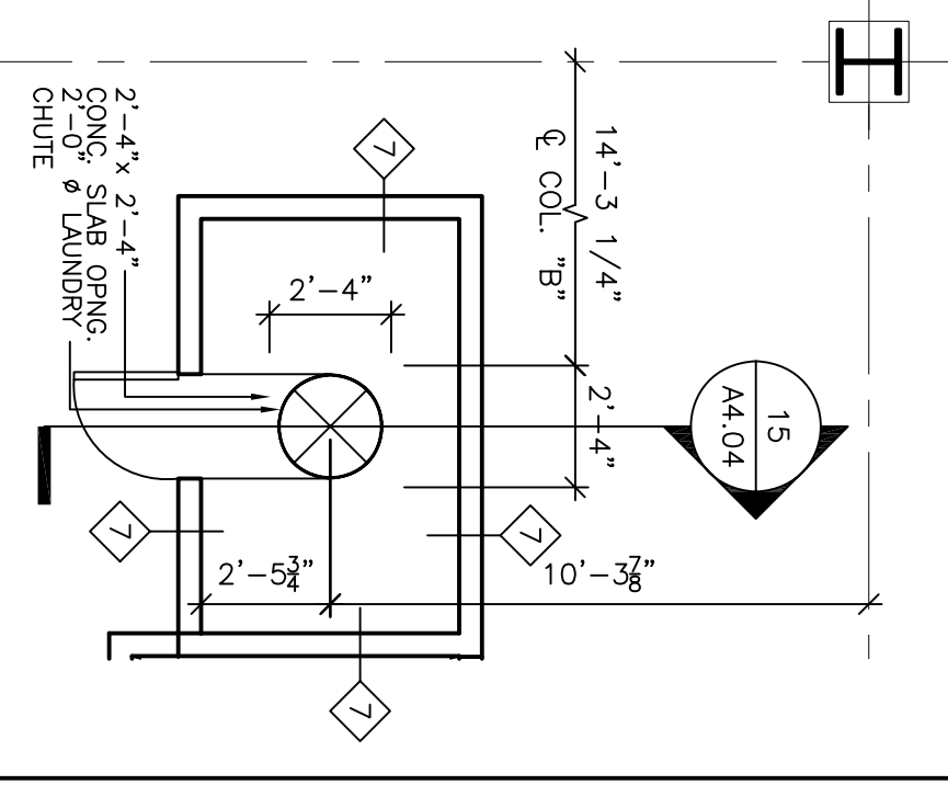
11 LAUNDRY CHUTE THIRD FLOOR SCALE: 1/4"=1'-0"
