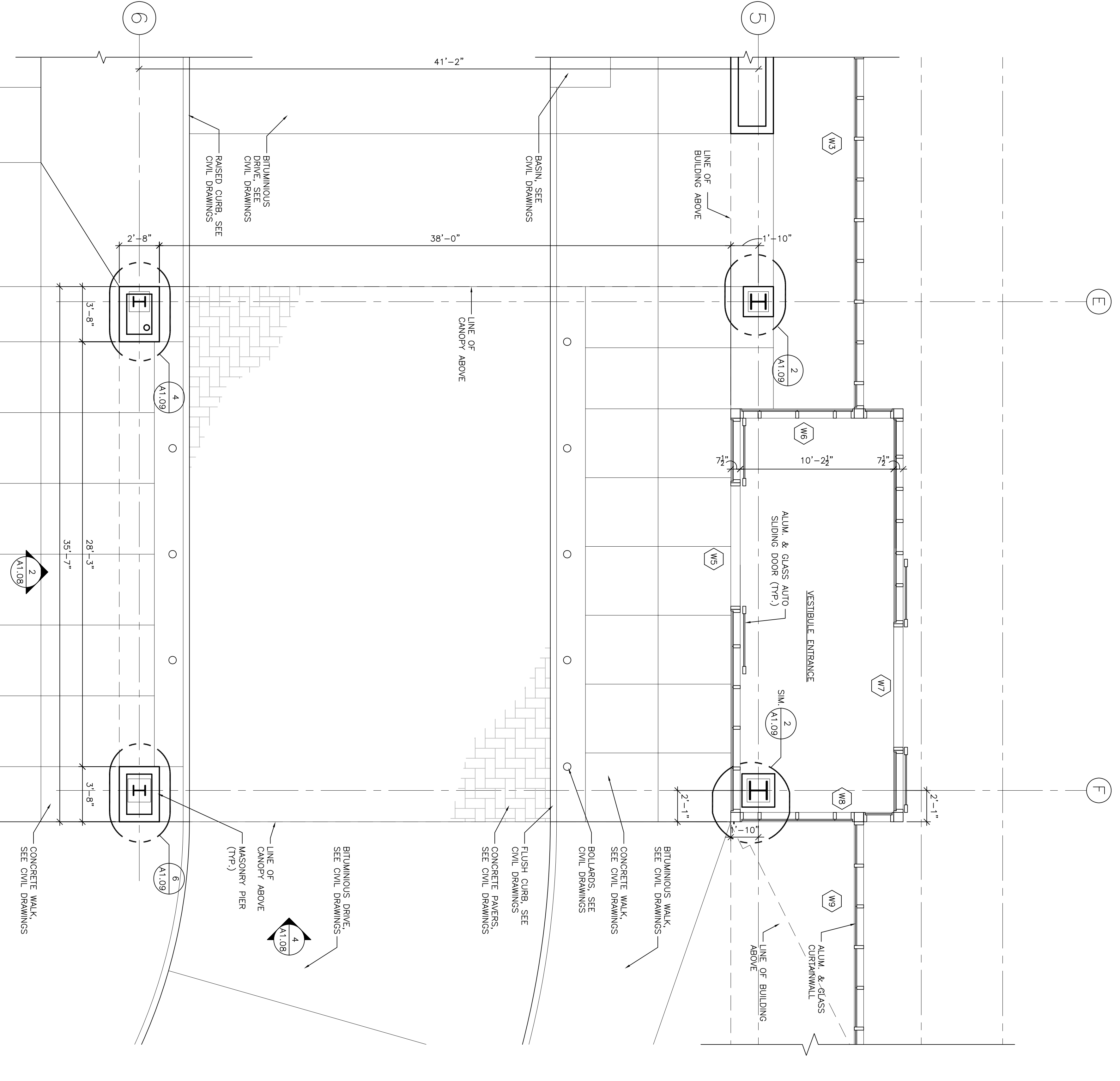
1 ENTRANCE CANOPY - PLAN SCALE: 1/4"=1'-0"
