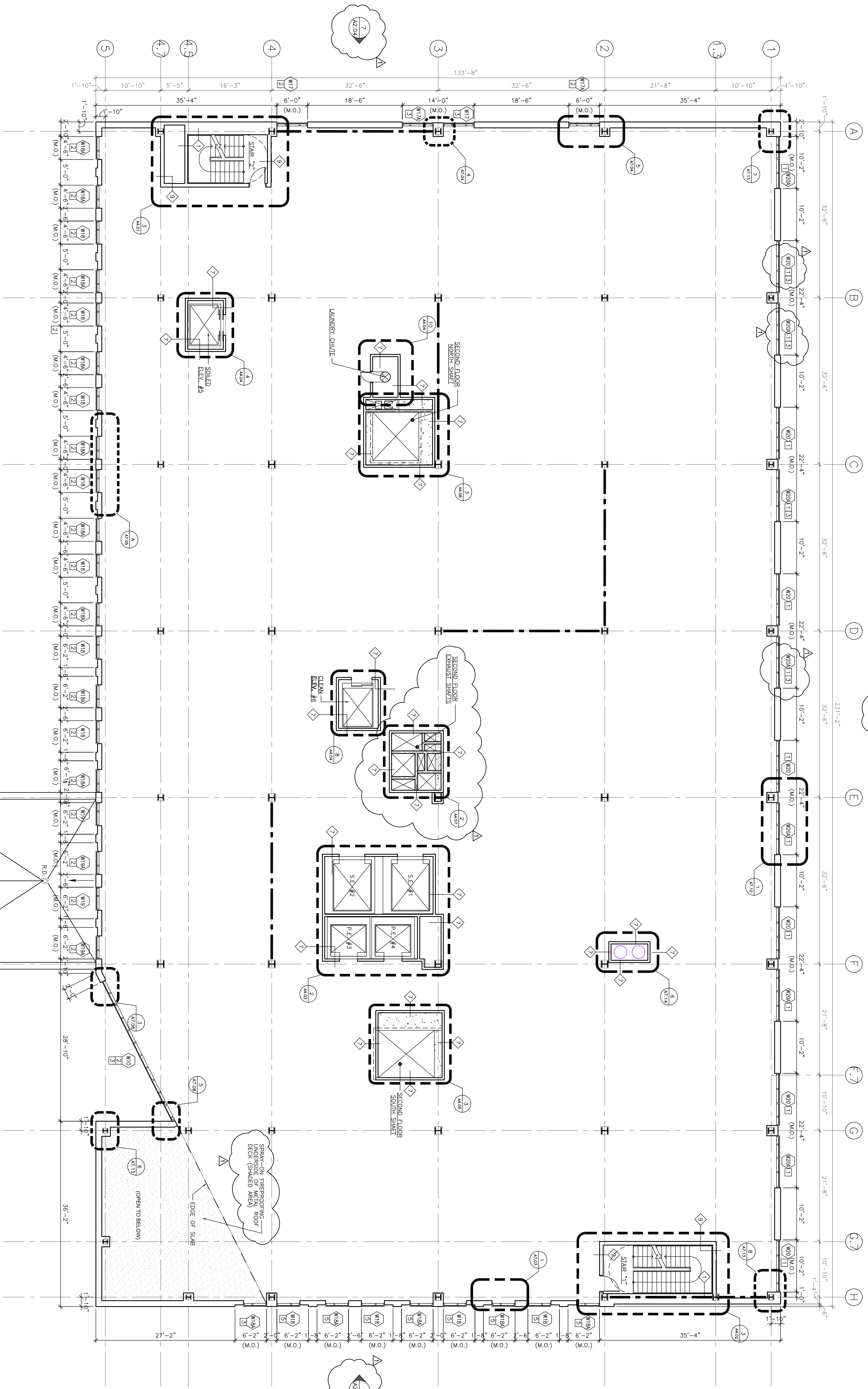
1 SECOND FLOOR PLAN SCALE: 1/8"=1'-0"
