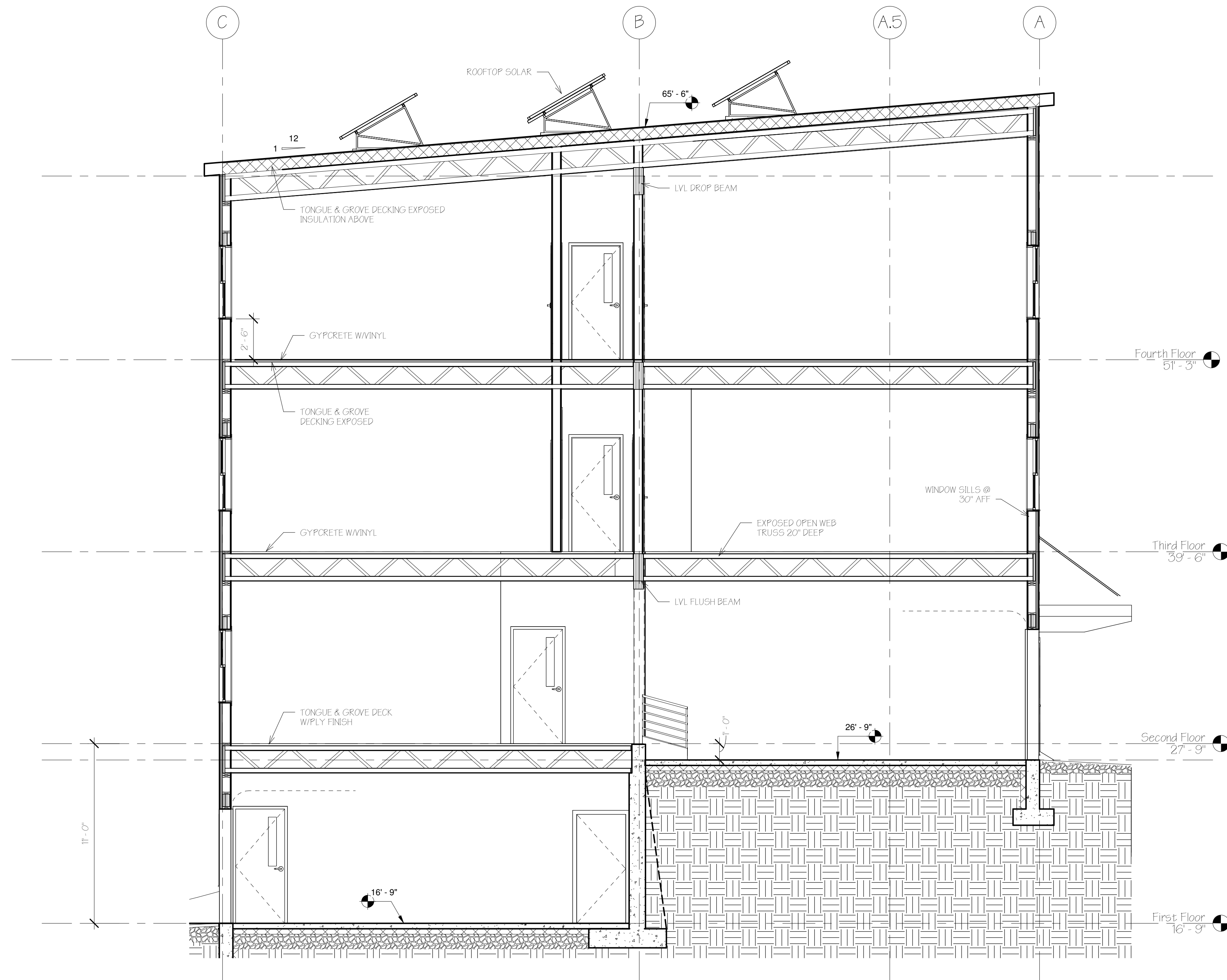
Ⓐ BUILDING SECTION 1/4" = 1'-0"
