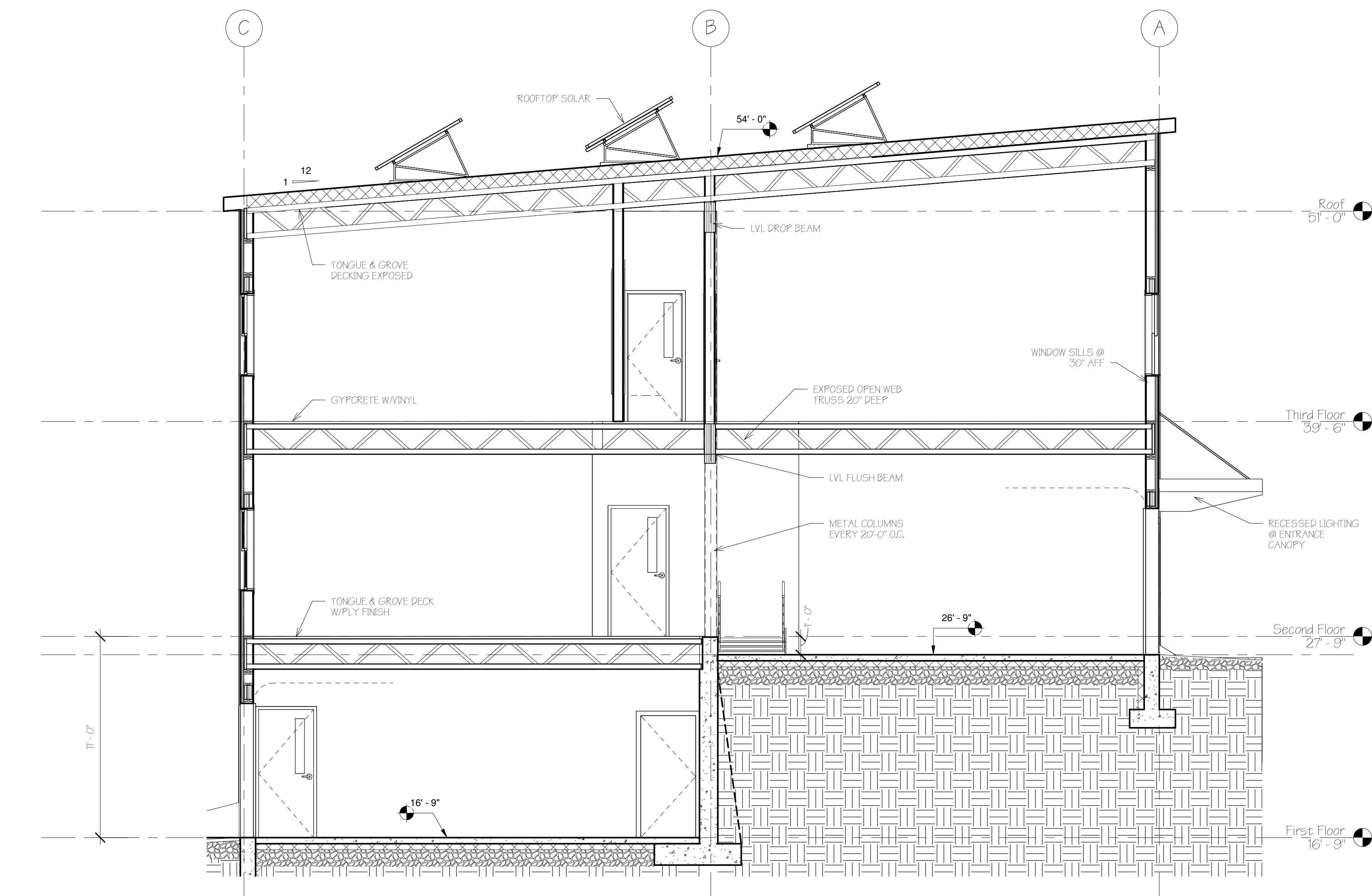
A BUILDING SECTION 1/4" = 1'-0"
