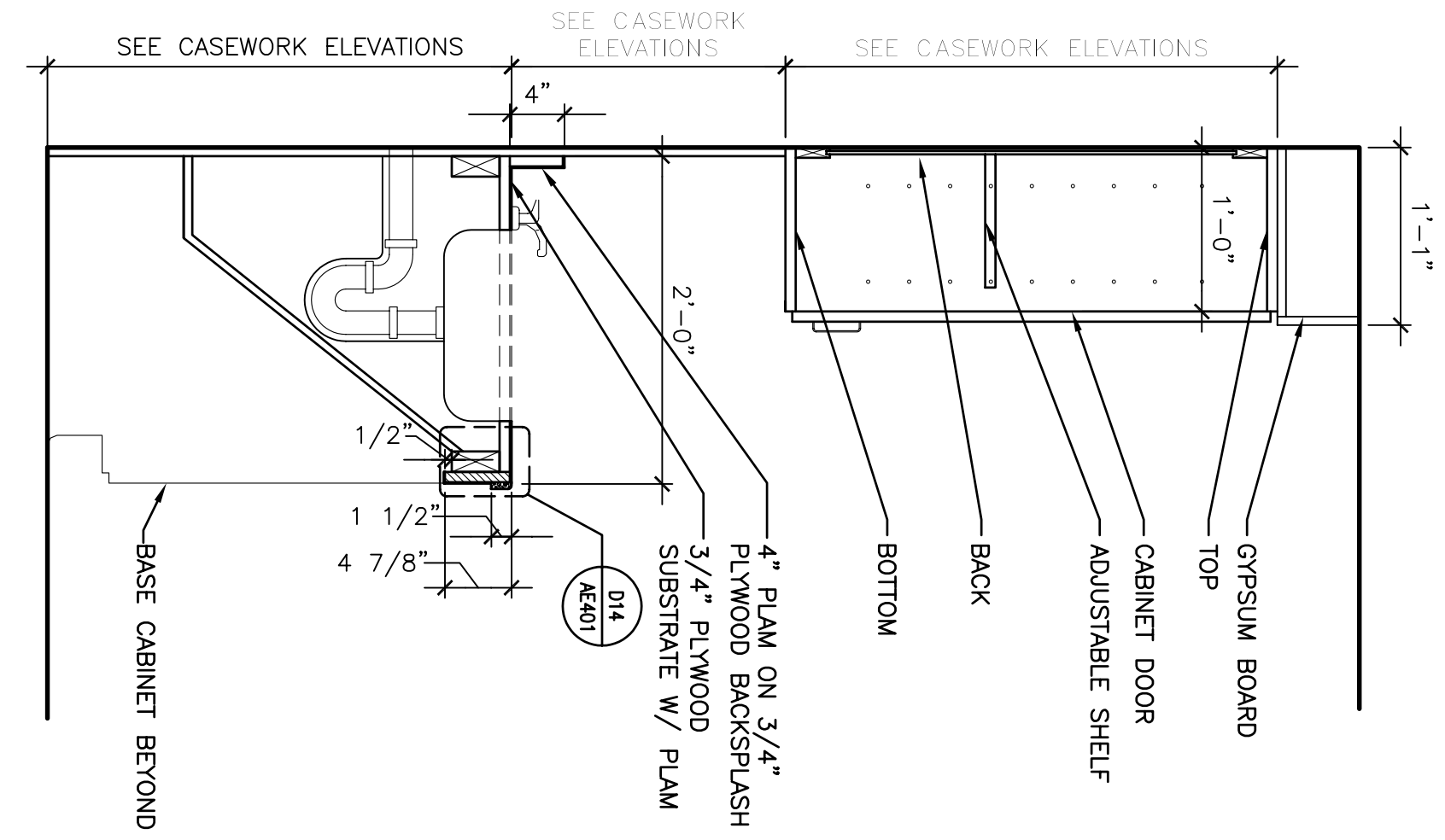
H14 CASEWORK SECTION
