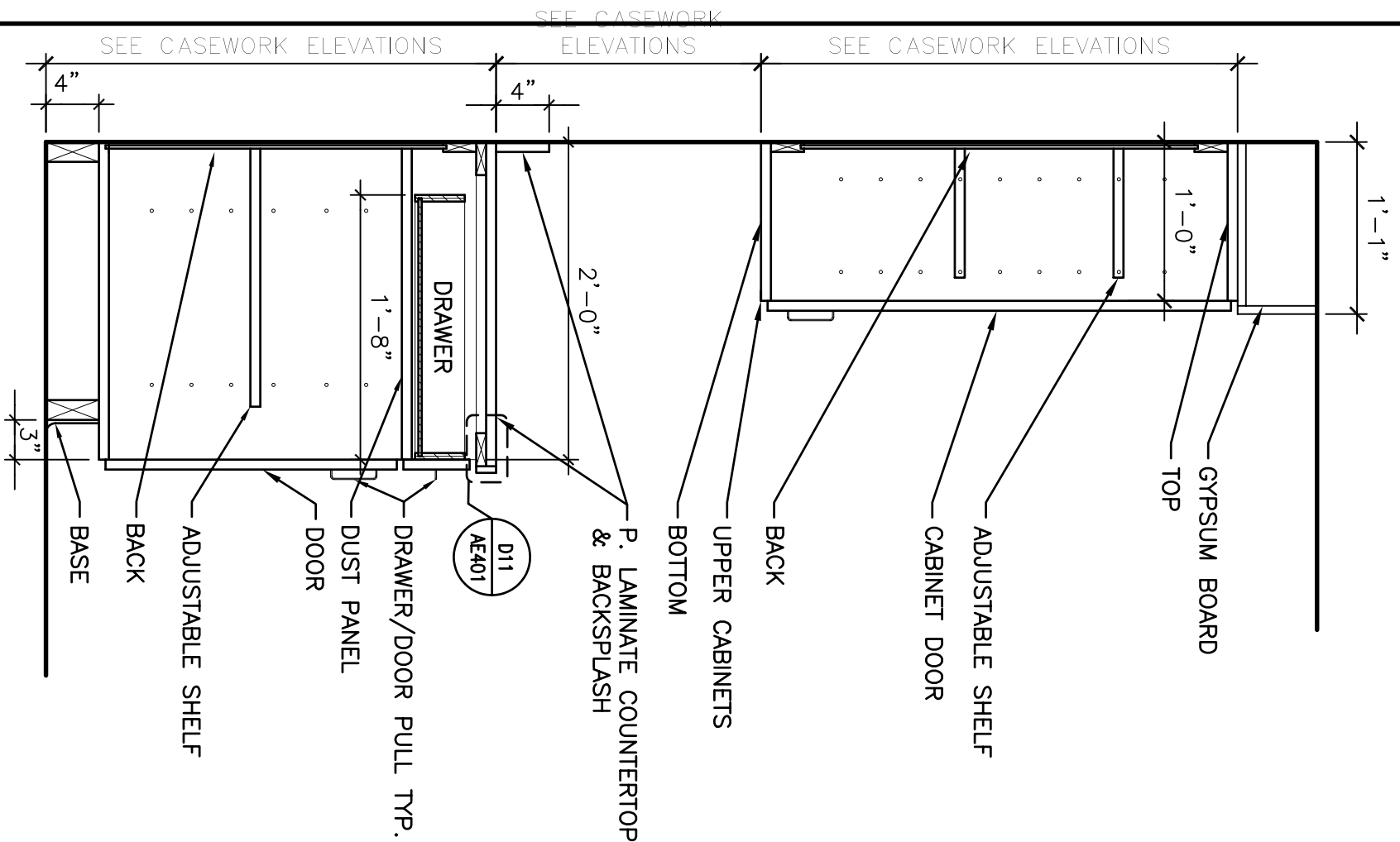
H11 CASEWORK SECTION
