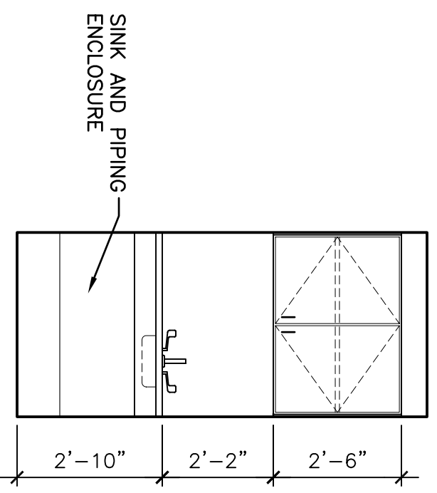
D1 INTERIOR ELEVATION CONFERENCE ROOM 20
