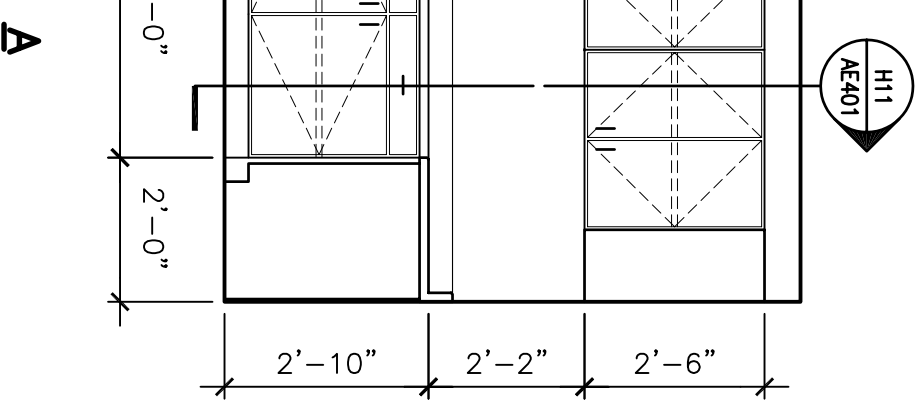
A1 INTERIOR ELEVATION - BREAK ROOM 16
