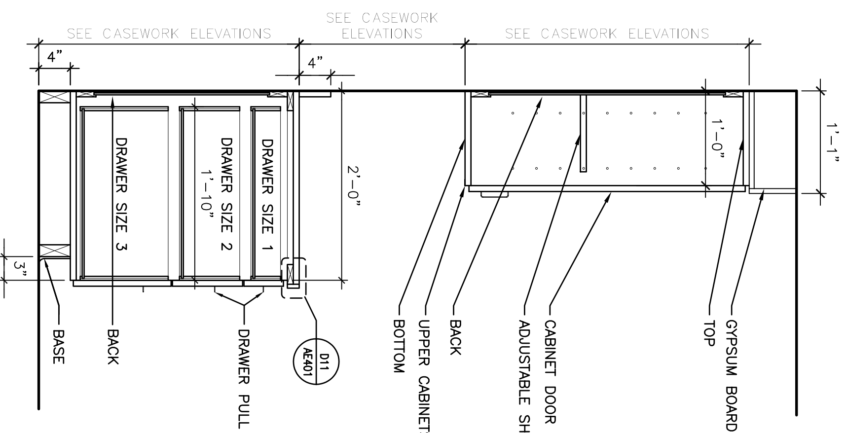
H9 CASEWORK SECTION
