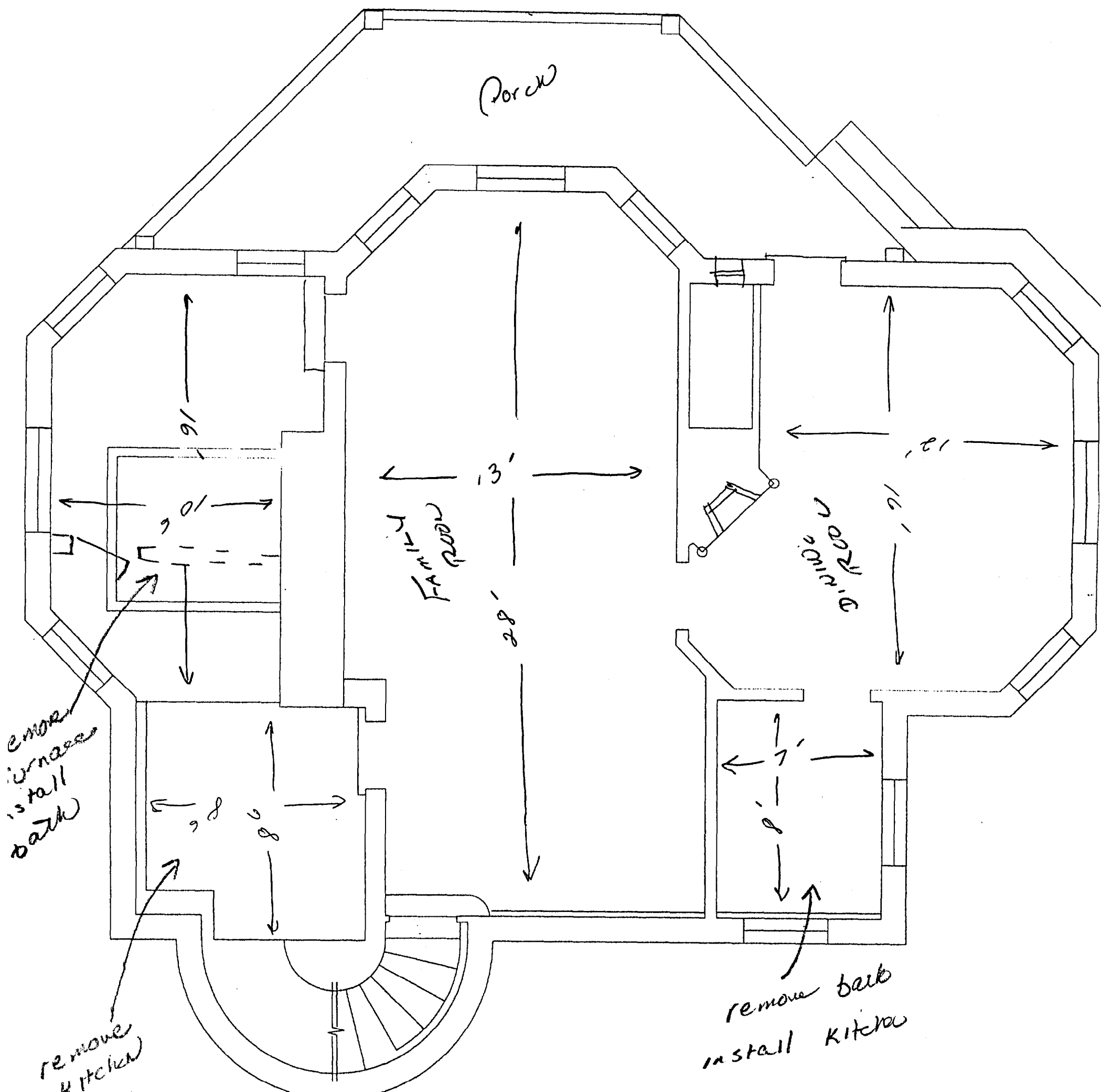
GROUND FLOOR
