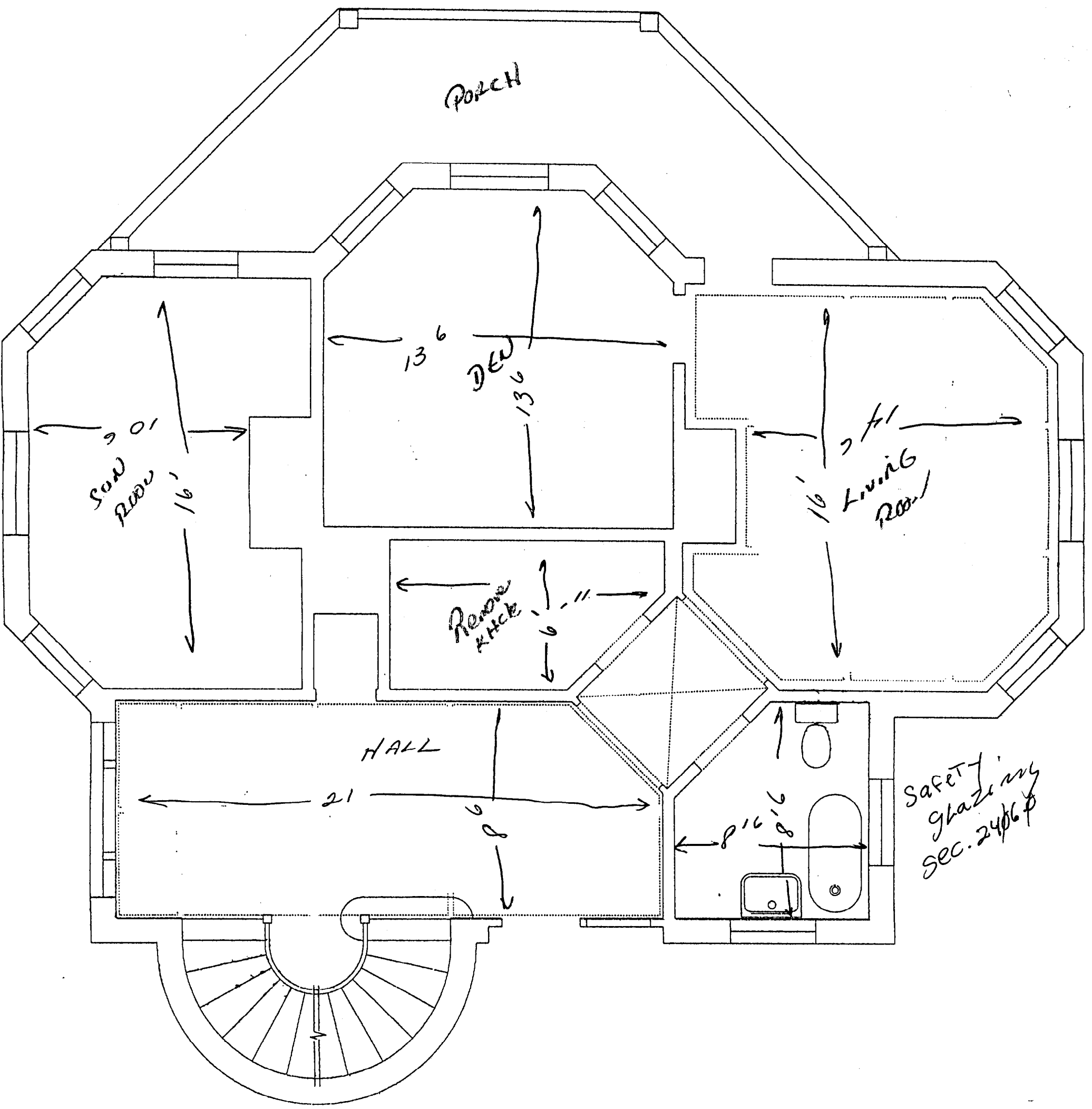
FIRST FLOOR
