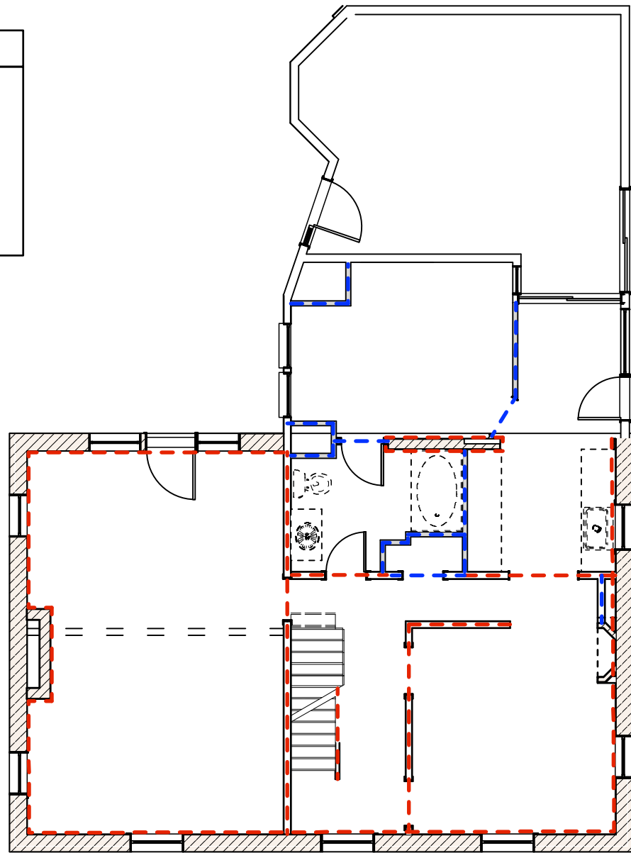
2 First Floor Interior Demo Plan Scale: 1/8" = 1'-0"
