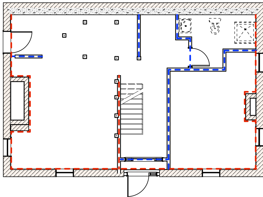
1 Basement Interior Demo Plan Scale: 1/8" = 1'-0"
