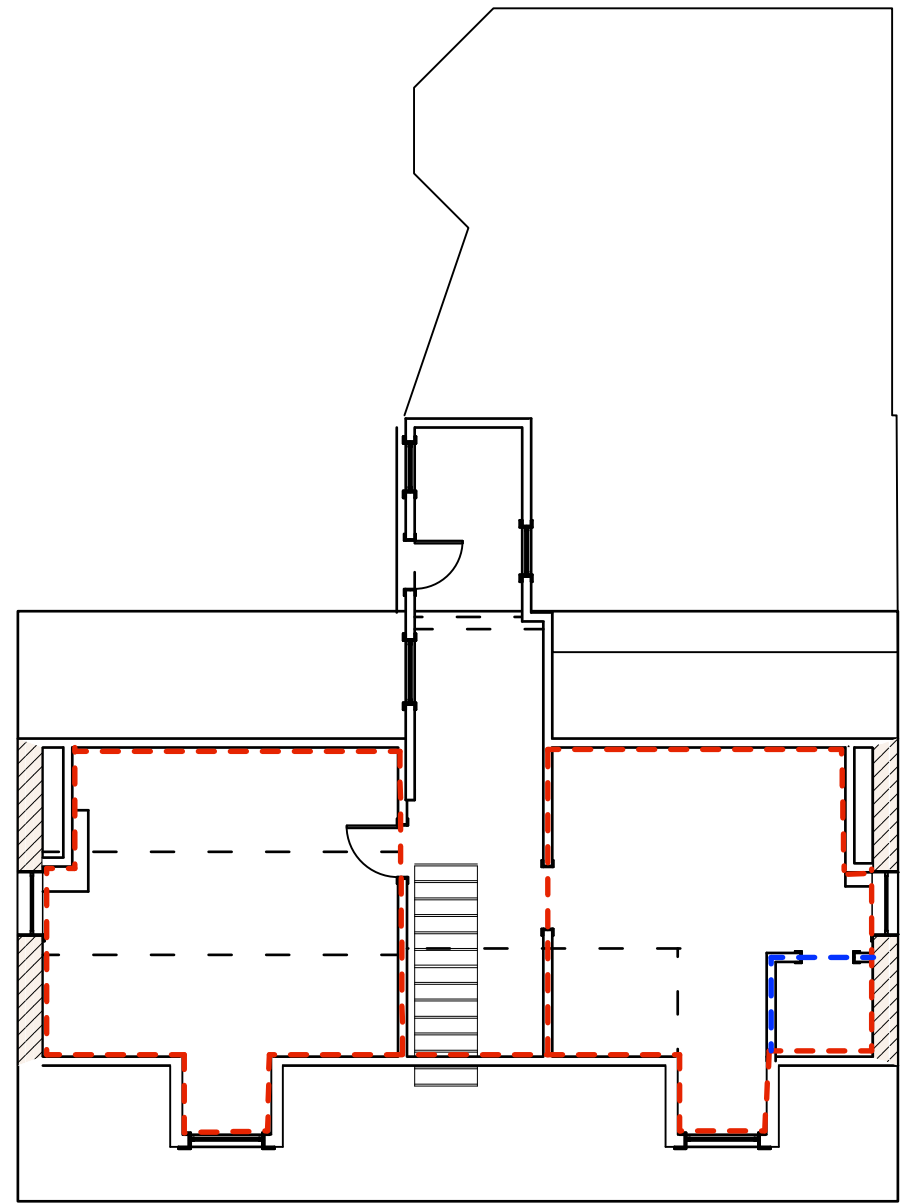
3 Second Floor Interior Demo Plan Scale: 1/8" = 1'-0"
