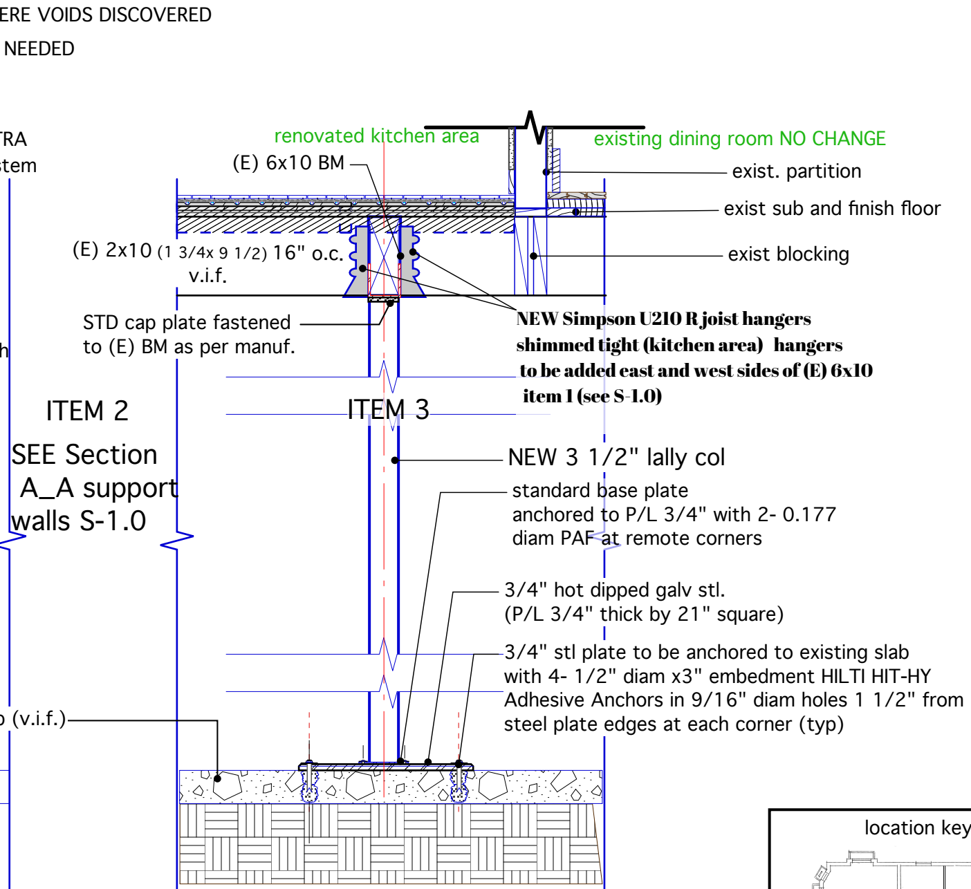
2. Section at kitchen/basement Lally Col
