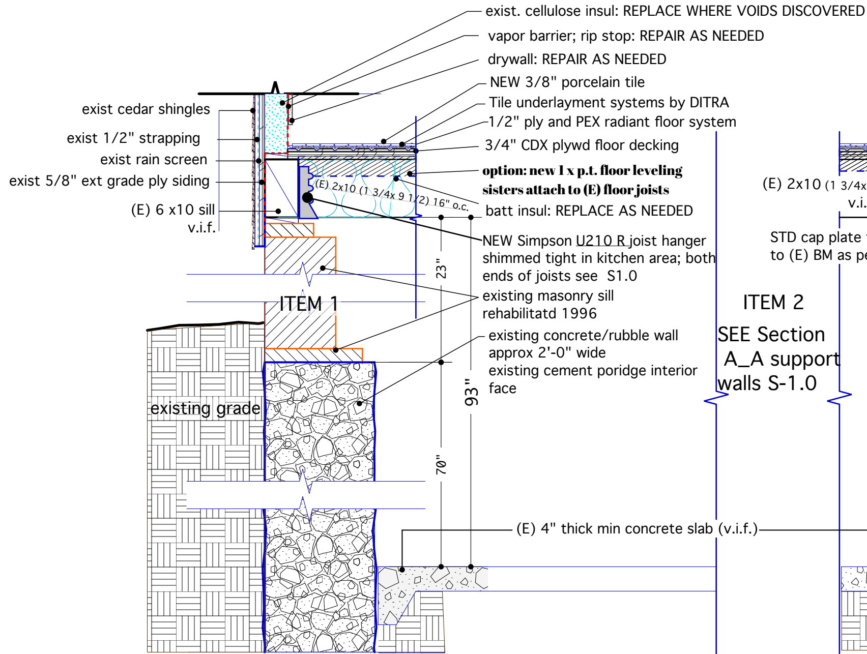
1. B/B revised EAST exterior section at kitchen/basement
