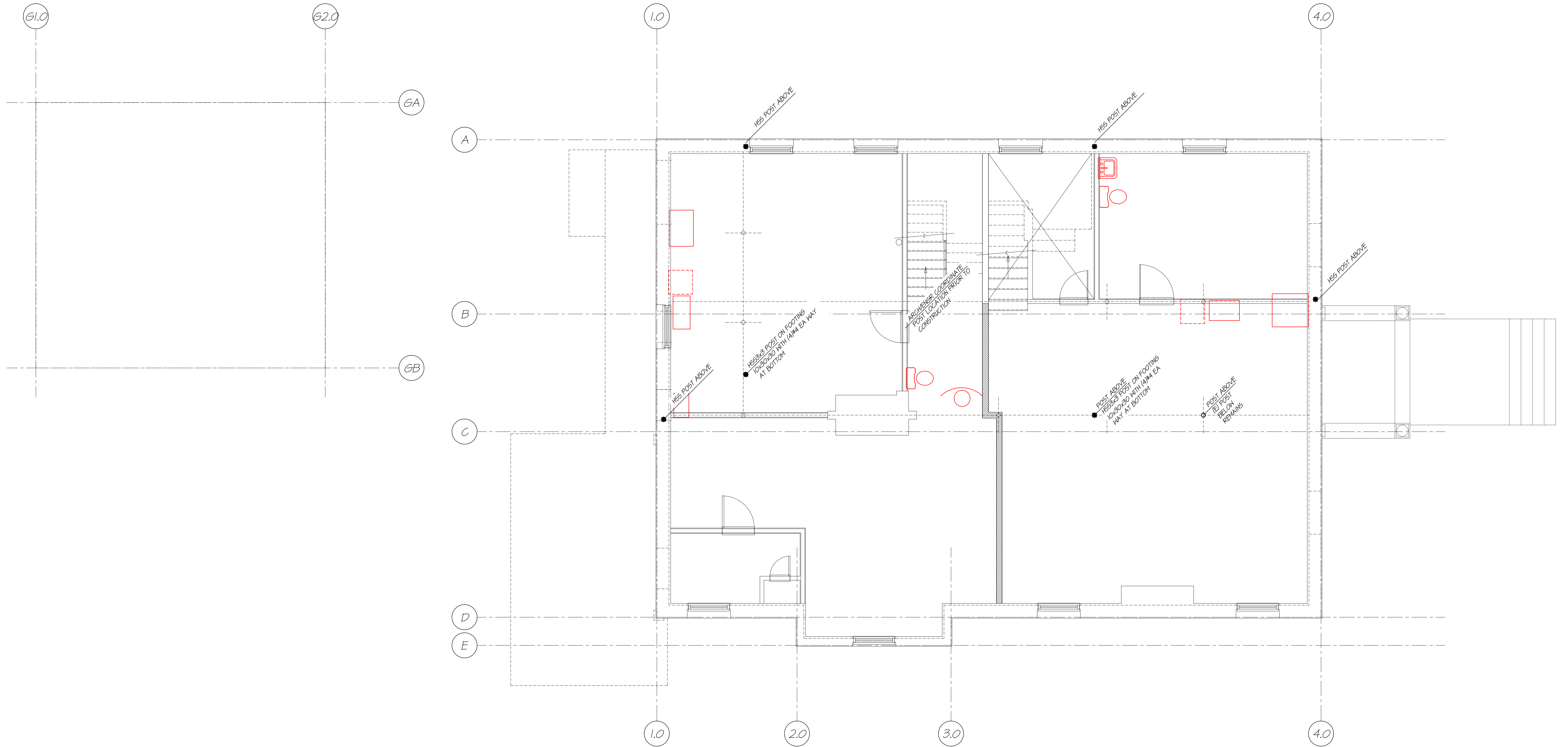
FIRST FLOOR FRAMING / FOUNDATION PLAN 1/4" = 1'-0"
