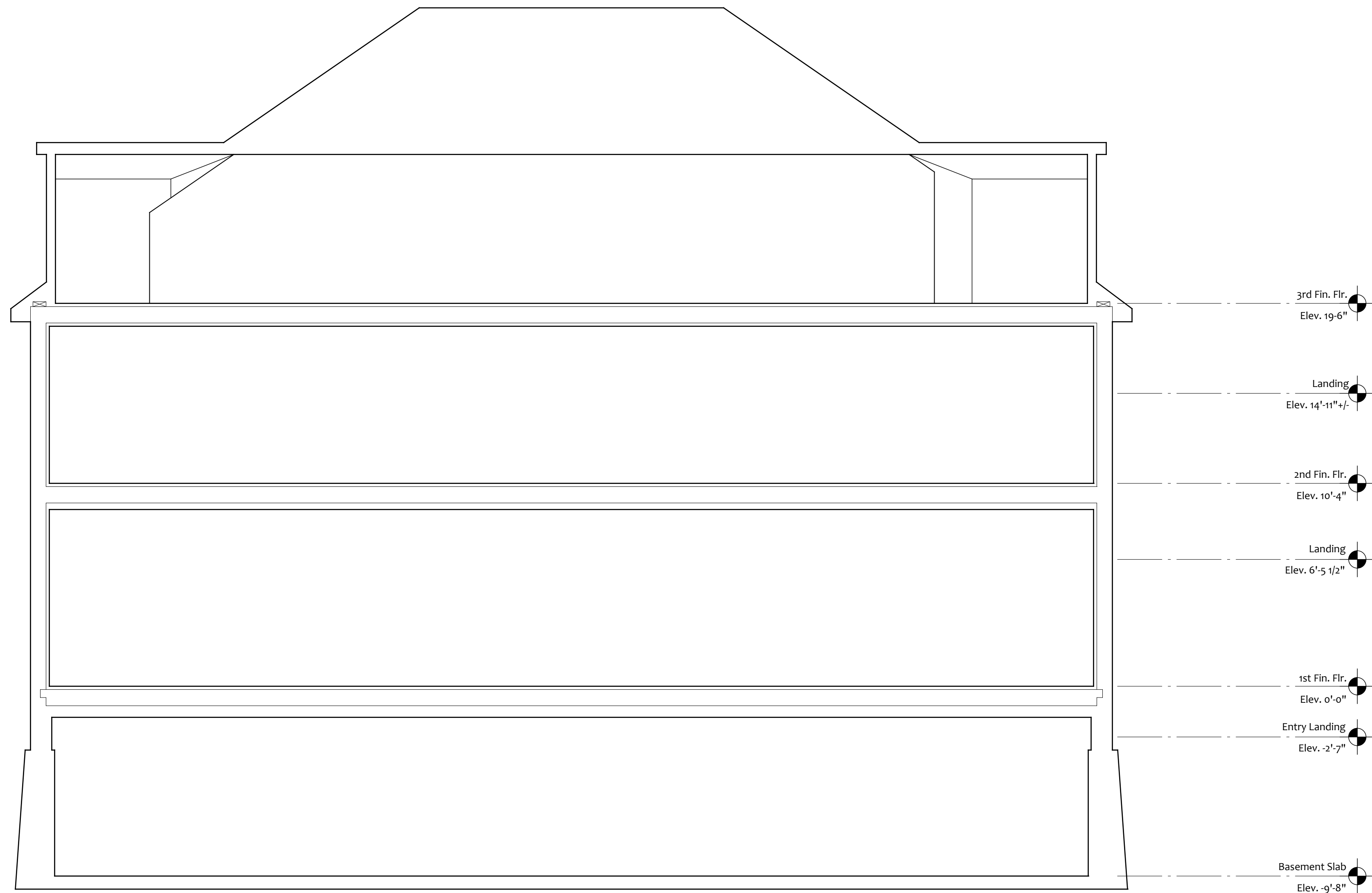
2 Building Section
