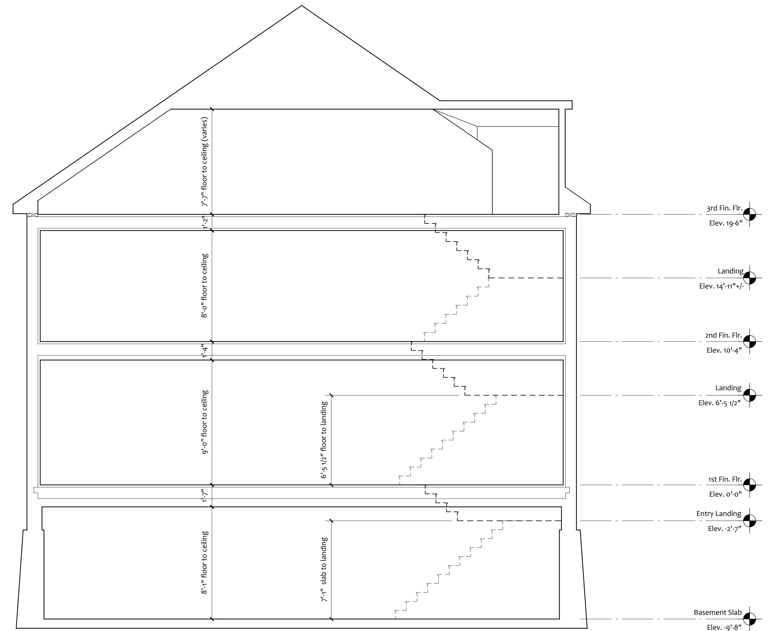
1 Building Section
