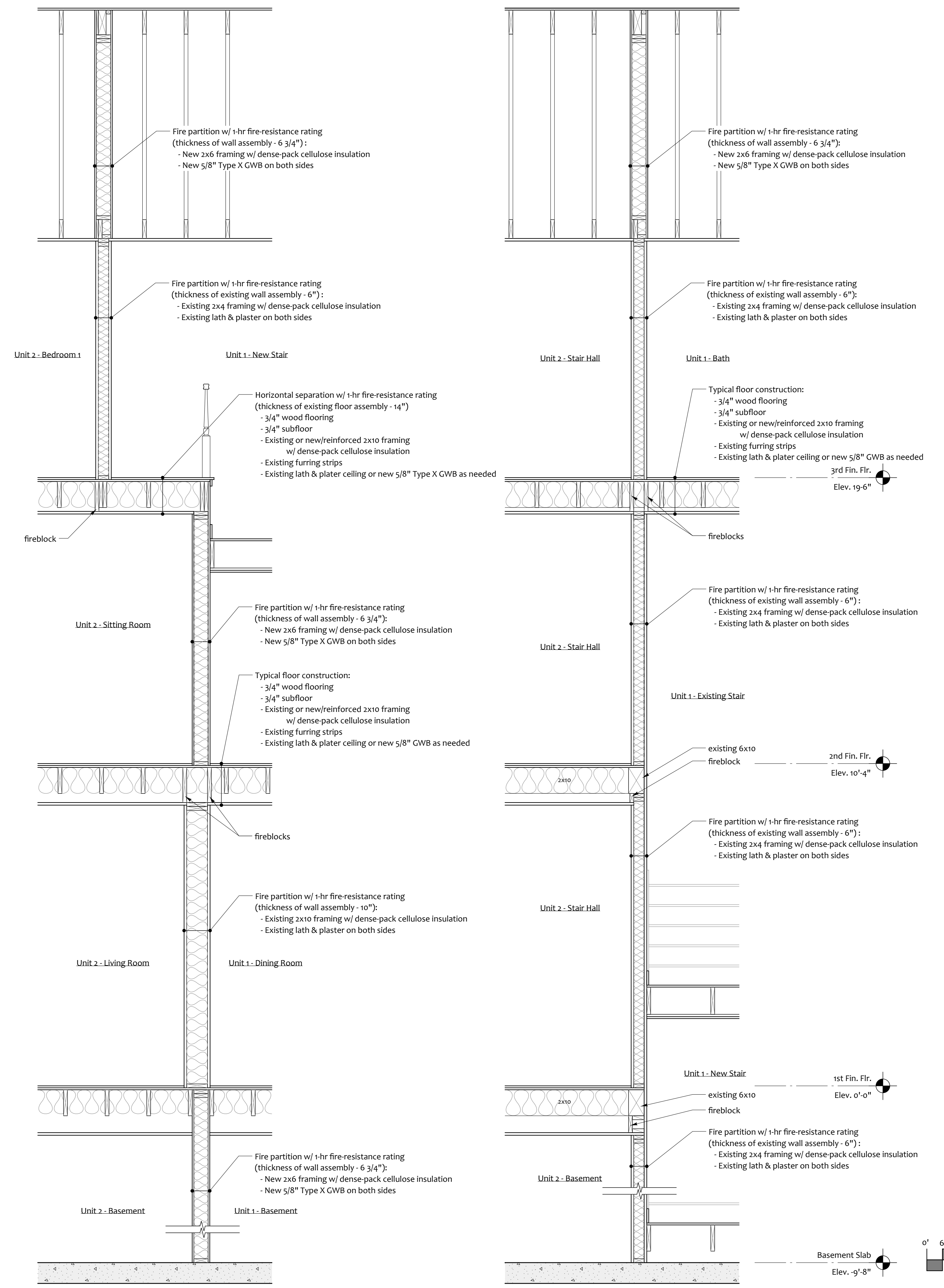
2 Wall Section
