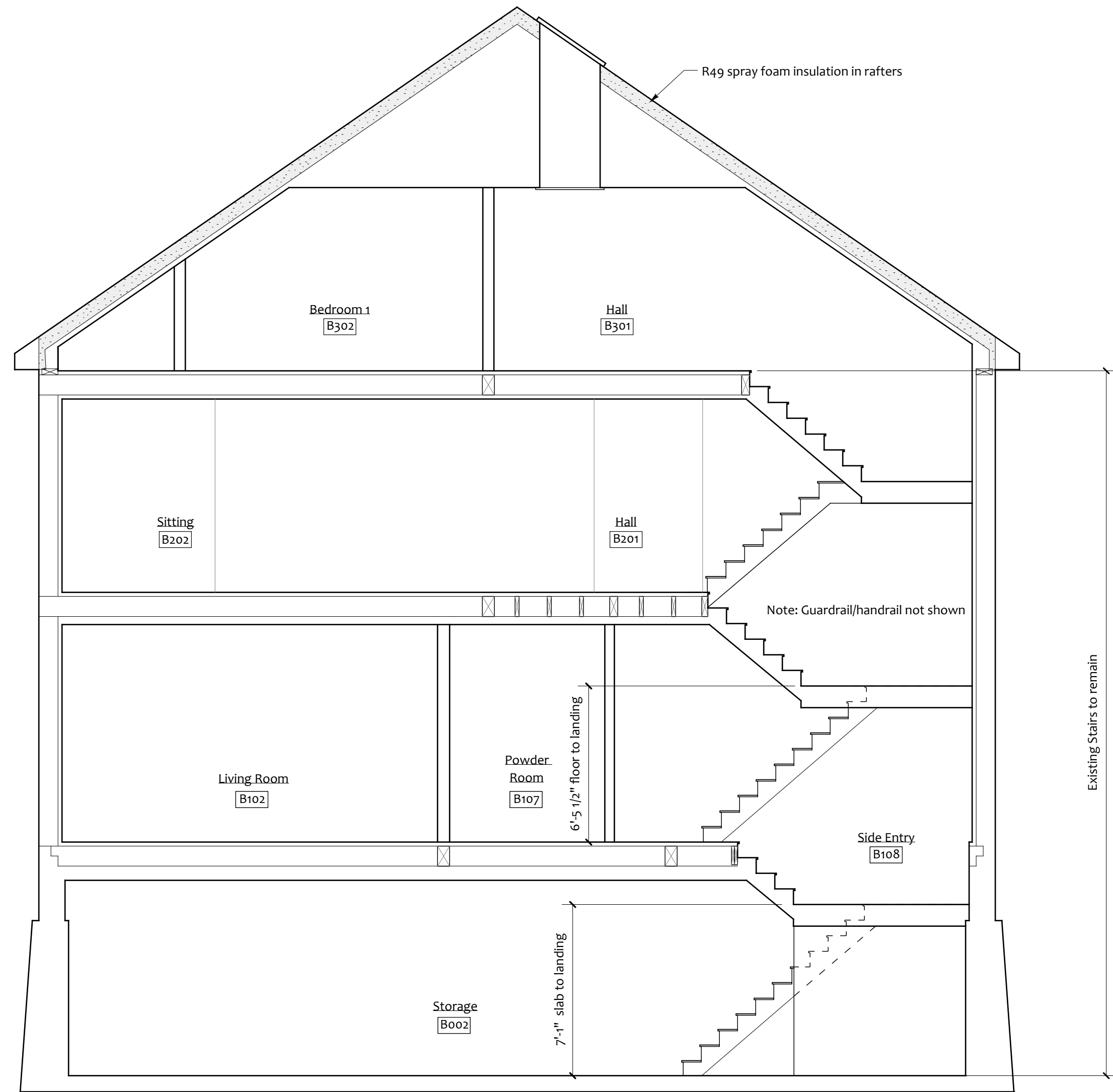
2 Building Section
