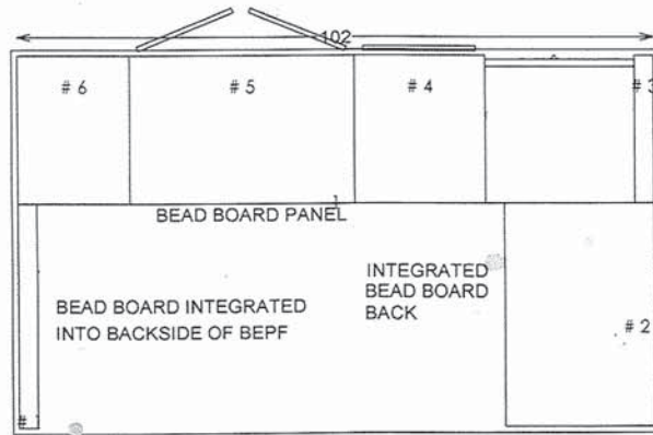
TRIM ISLAND WITH FLAT STOCK
