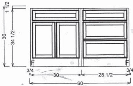
ELEVATION B WAINSCOT PANEL
